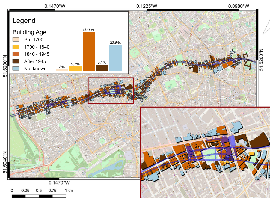
FIGURE 8 Age-based classification of the buildings between Paddington and Liverpool Street, along the Crossrail twin tunnels in central London. The Crossrail alignment is represented with a blue line
