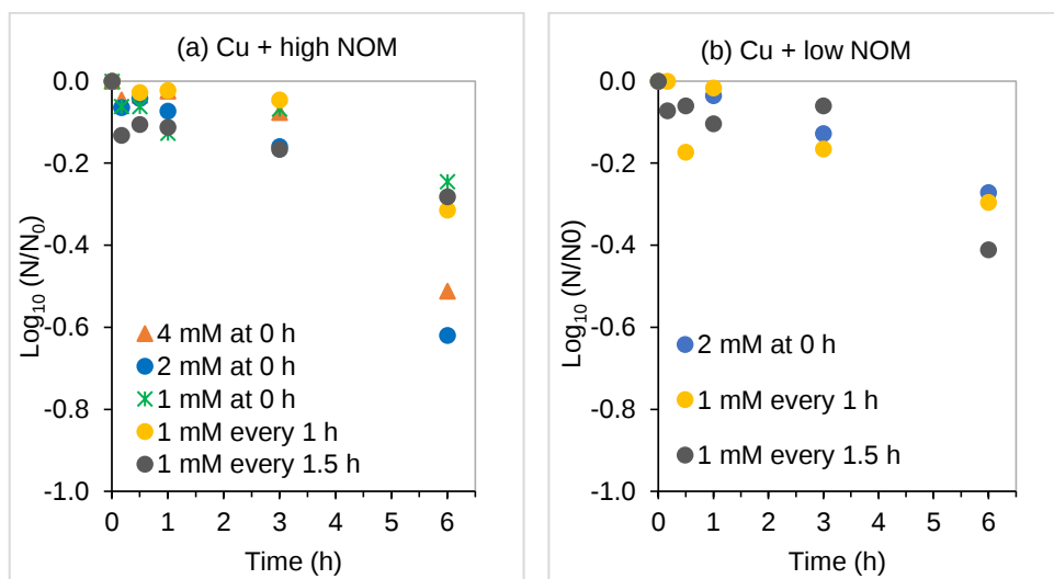
Figure 4-9 \text{Log}_{10} inactivation of PhiX 174 by Cu in (a) high NOM water (20 mg C/L) or (b) low NOM water (2 mg C/L) using different doses of tempol at different times (see legend).
