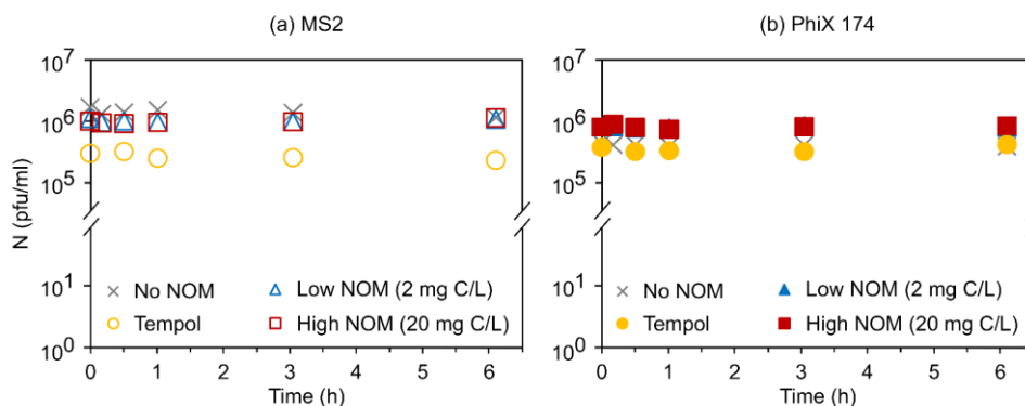
Figure 4-10 Stability of (a) MS2 and (b) PhiX 174 bacteriophage in all water matrices used (no NOM, low NOM, high NOM and with tempol).
