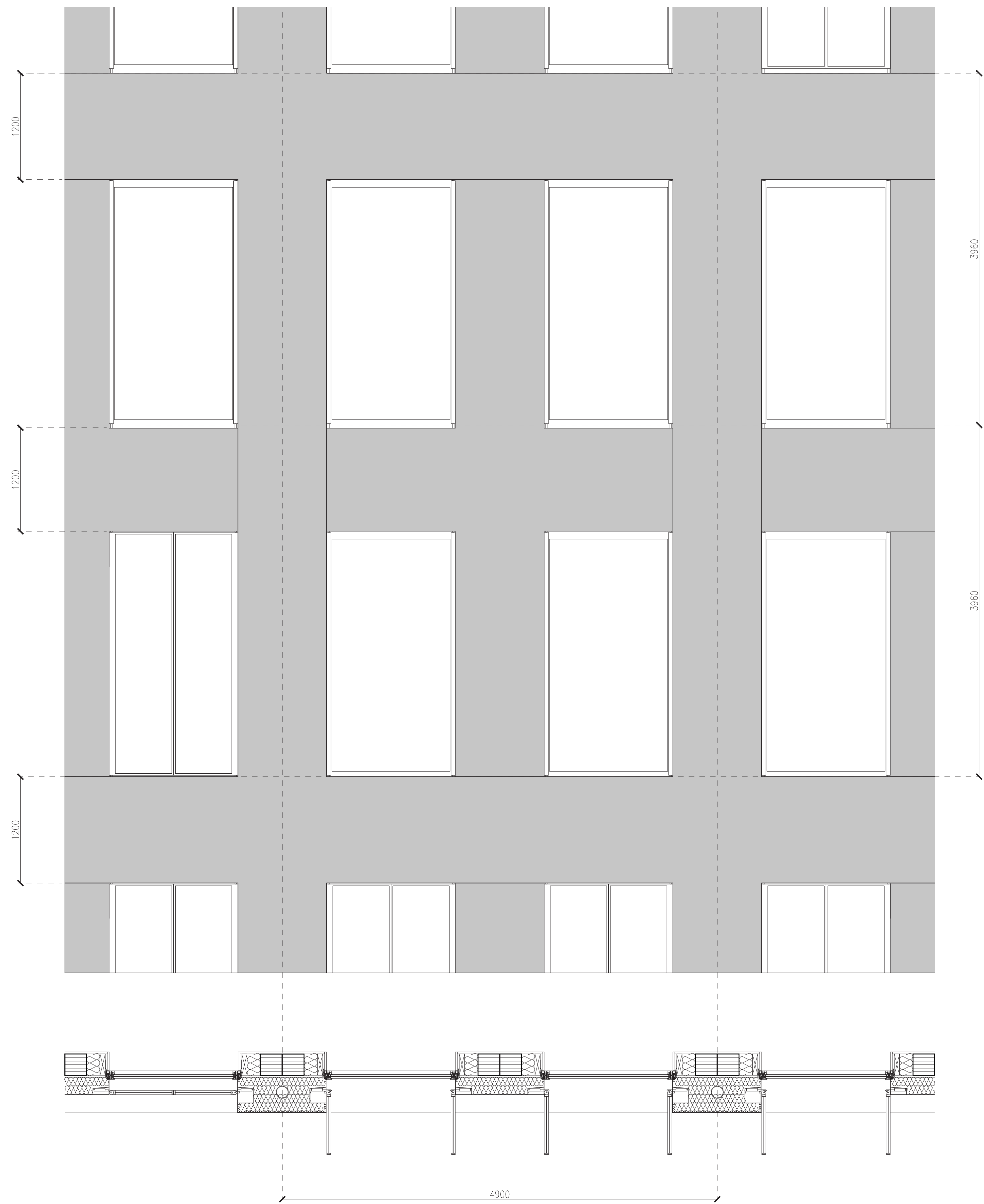
ENVELOPE - TOWER ADAPTABLE FLOORS - 1:20
