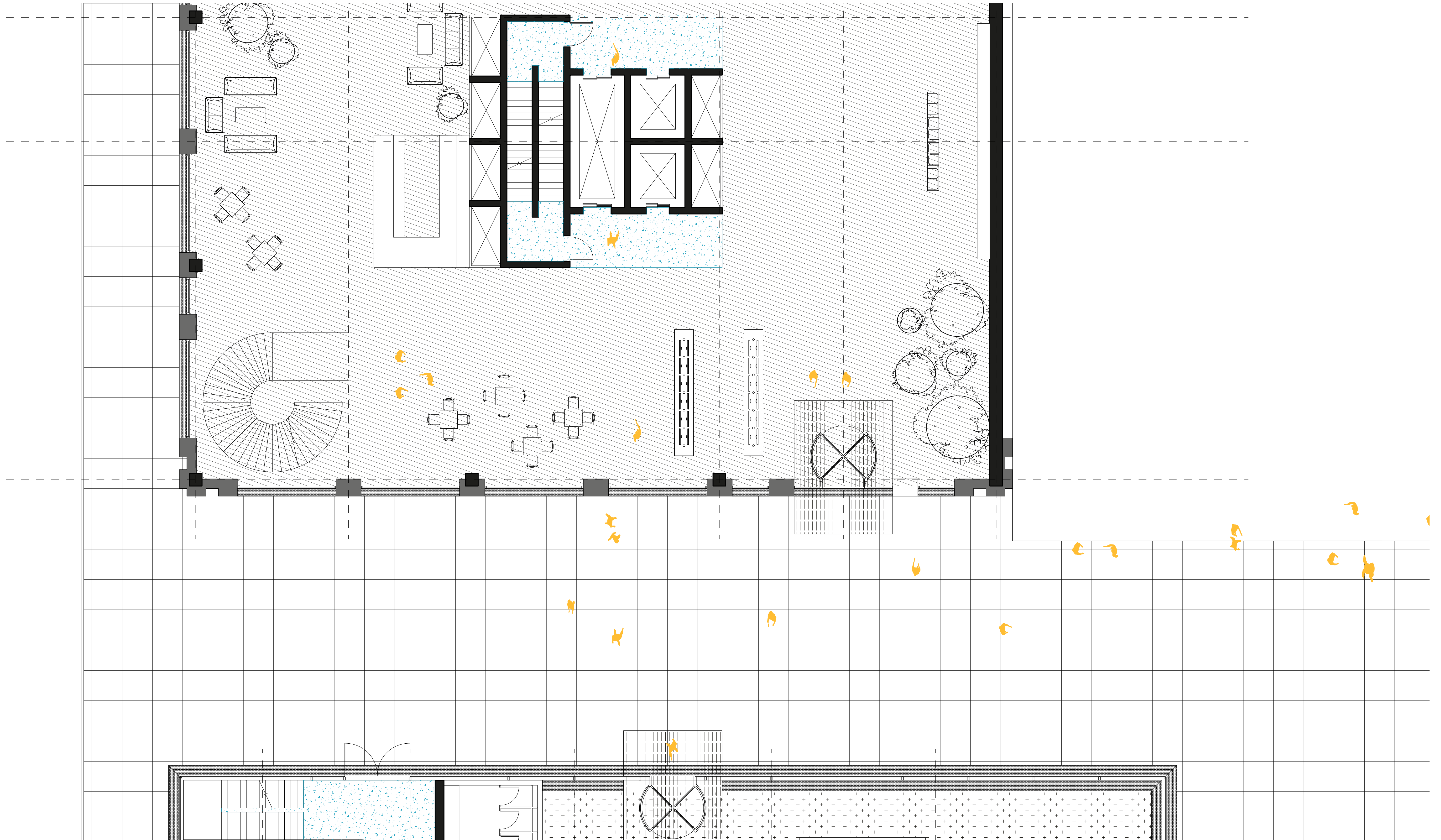
FRAGMENT - LOBBY & COMMUNITY FUNCTION ADJACENCY- 1:50
