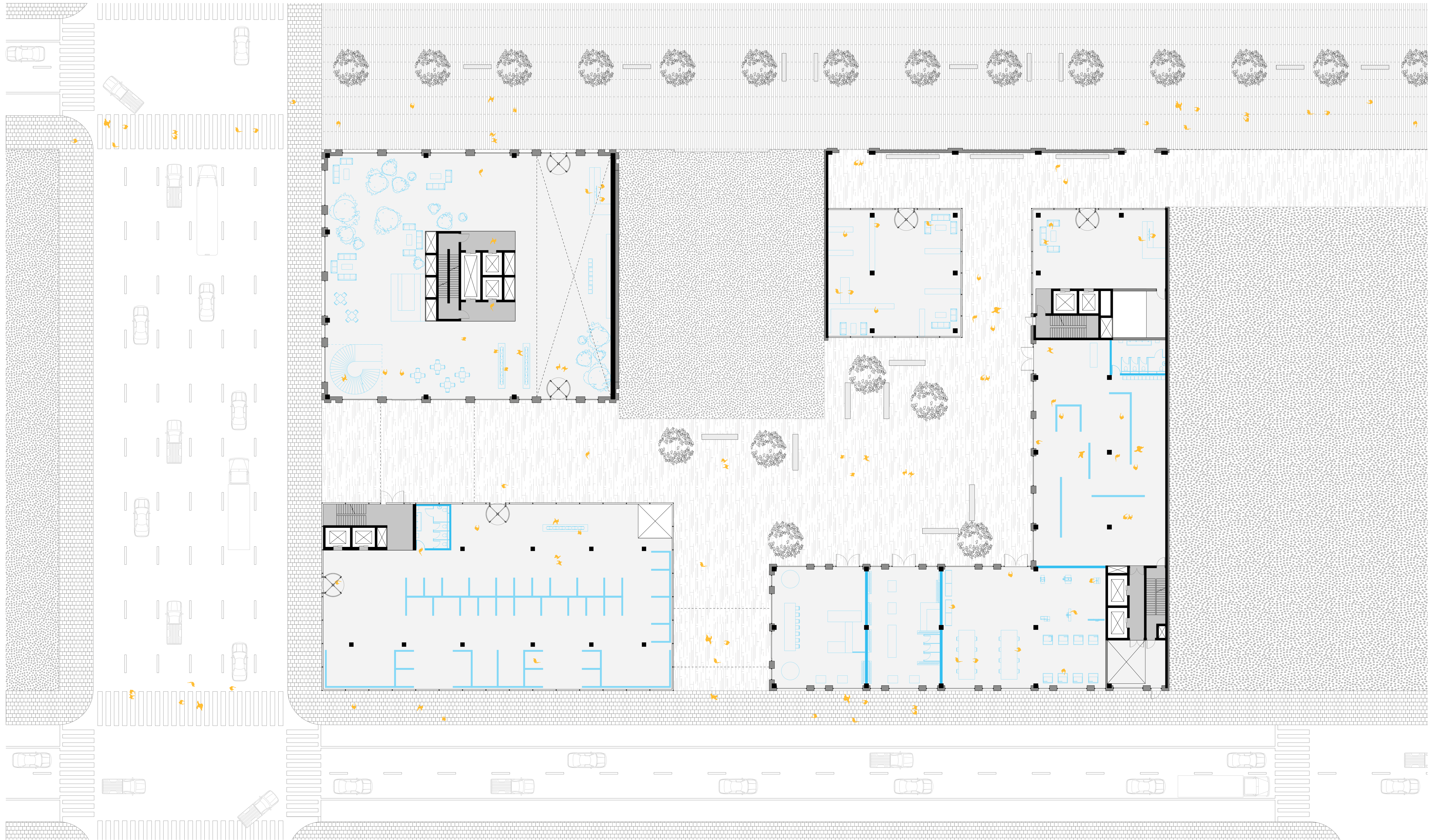
GROUND FLOOR - LOADED - ALTERNATIVE 1:200
