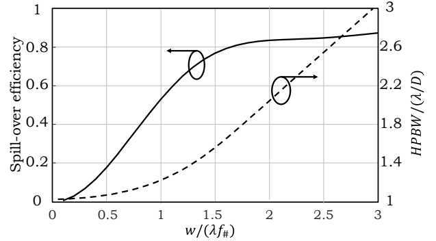
Fig. 7. Spill-over efficiency (solid) and HPBW (dash) for an ideal absorber under an optical system characterized by f_\# = 2 and diameter D = 100\lambda versus the physical size of the absorber normalized to \lambda f_\# .
