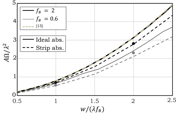
Fig. 10. Normalized throughput calculated as \eta_{ap}/\eta_f versus the absorber size, w , for two optical systems with f_{\#} = 0.6 (grey) and f_{\#} = 2 (black). The solid lines are related to the ideal absorbers, the dashed lines to an absorber based on resistive strips, and the dots to the relevant performed full wave simulations.
