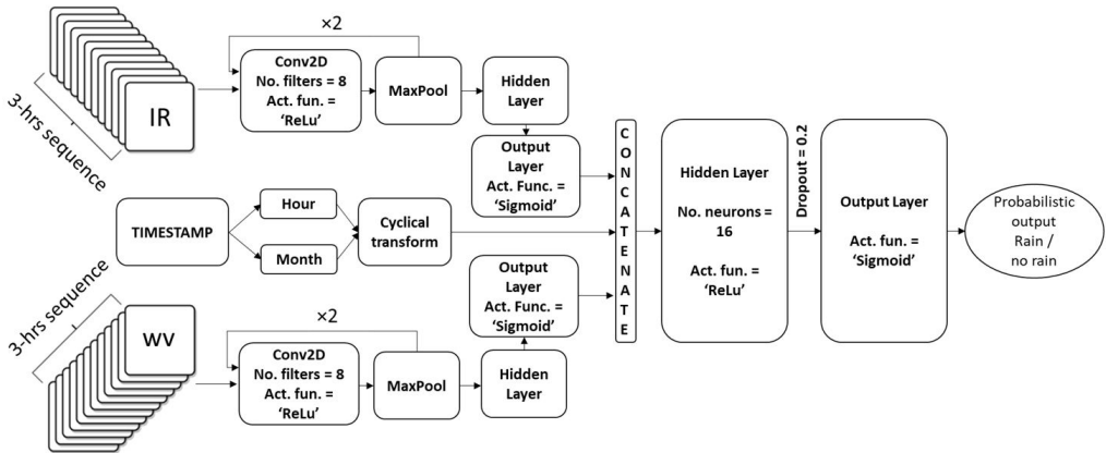
Figure 3.4: Schematic overview of the proposed bispectral (WV + TIR) RainRunner architecture.
