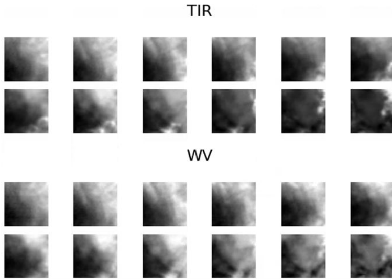
Figure 4.14: Example of a case when the addition of WV information corrected false alarms of the TIR-only model. Station TA00405 on the 20th of June 2019.
