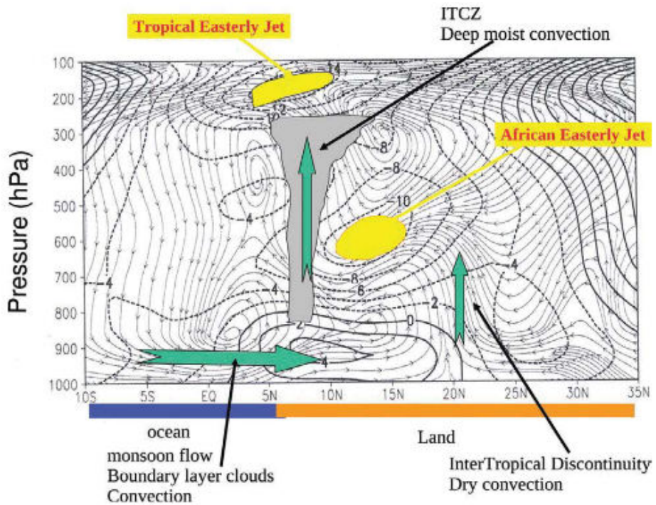
Figure 4.16: Mean Meridional Circulation (stream lines) and associated mean Zonal Wind (m/s in contours) over West Africa during the summer season [98].
