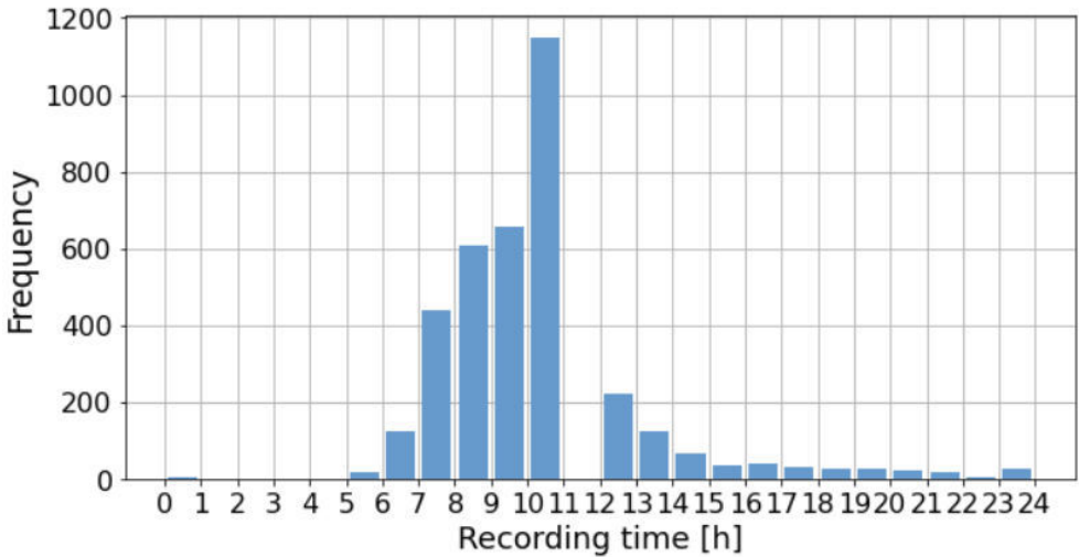
Figure 2: Distribution of citizen scientist recordings in time.
