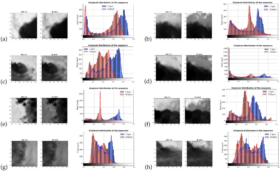
Figure 3: Dry intrusions observed at TAHMO locations. The characteristics of each dry intrusion are presented in Table 2.
