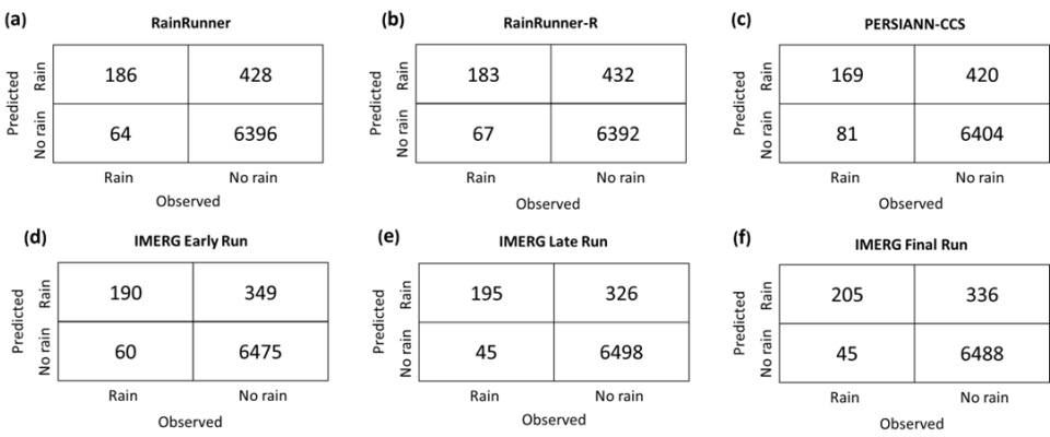
Figure 2.10: Contingency tables of (a) RainRunner, (b) RainRunner-R, (c) PERSIANN-CCS, and (d) IMERG Early, (e) Late, and (f) Final run on the independent test dataset, consisting of 250 rain and 6824 dry sequences.
