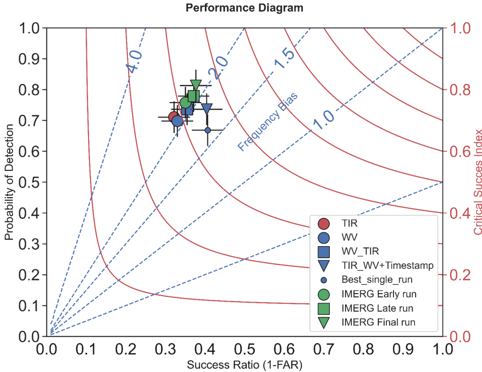
Figure 3.7: Roebber performance diagram on the test dataset.
