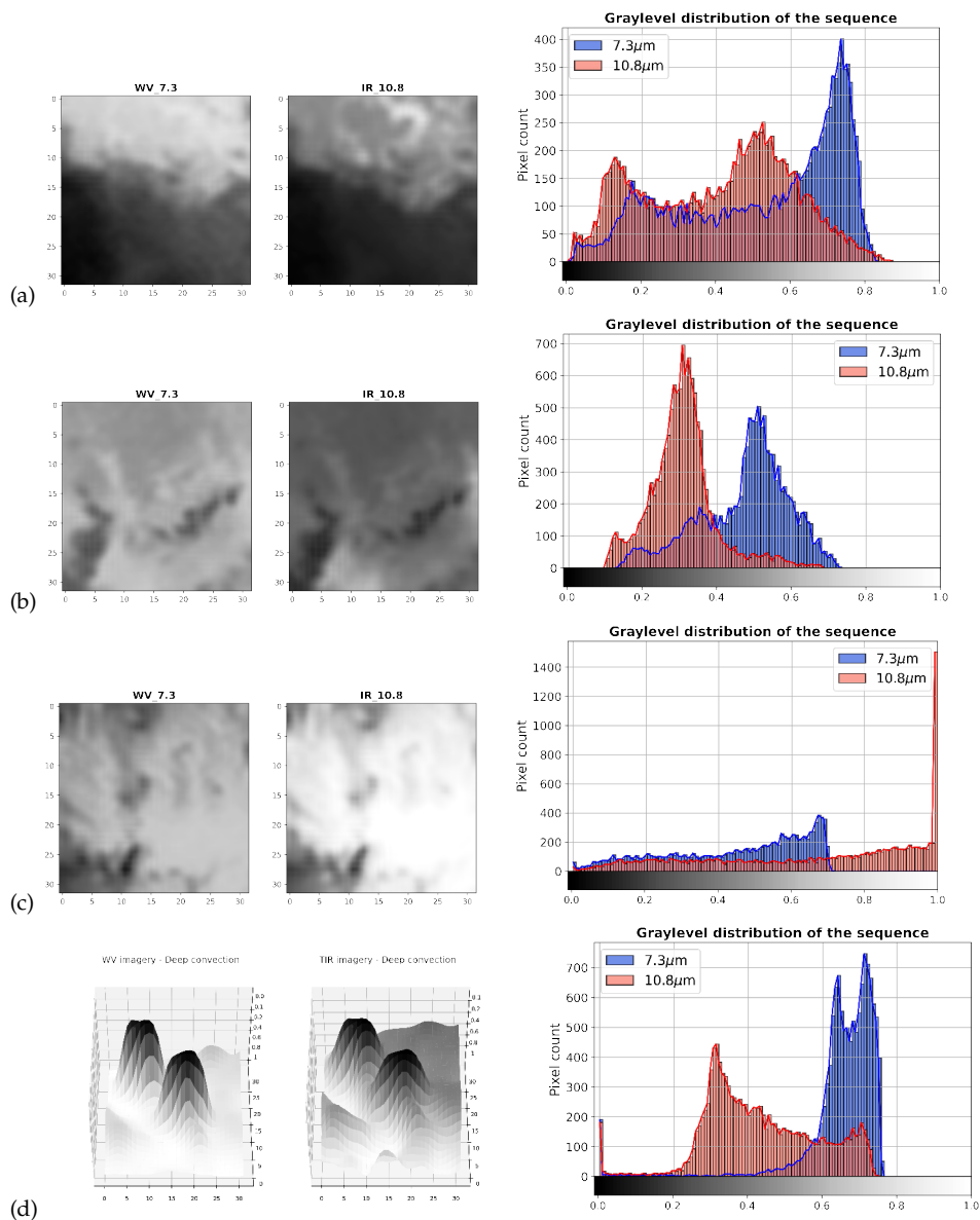
Figure 3.11: Pixel analysis of relevant atmospheric events: (a) dry intrusion from the North, (b) dry slot, (c) low-level moisture detected in WV, and (d) 3D deep convective motions of a heavy precipitation event as seen in WV and TIR imagery.
