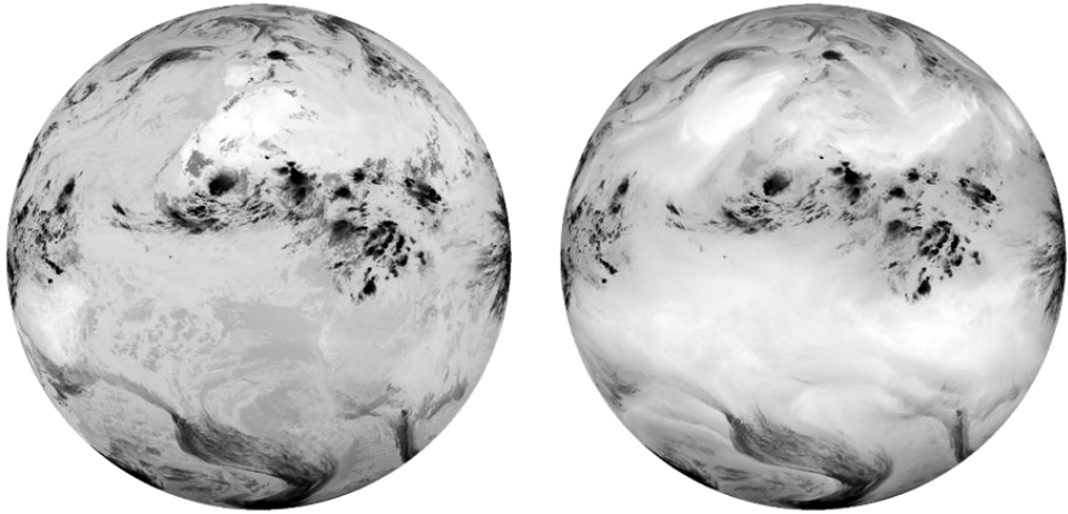
Figure 4.4: Images from the two MSG channels used in this study, on the 21st of August 2021 at 17:30 UCT. Left: Channel 9, 10.8 \mu\text{m} ; right: Channel 6, 7.3 \mu\text{m} .
