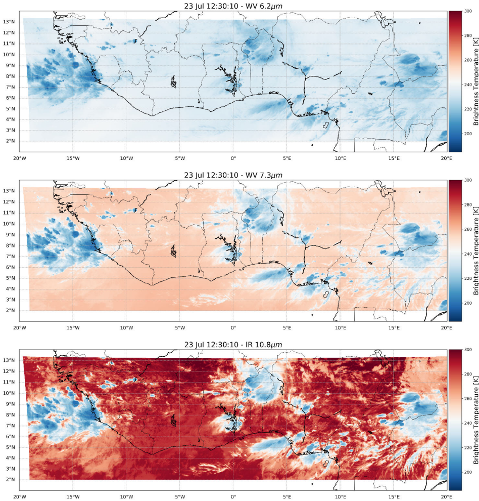
Figure 3.10: Data from the three considered SEVIRI infrared channels over West Africa on July 23 2020 at noon: from top to bottom: WV 6.2 \mu m (Channel 5); WV 7.3 \mu m (Channel 6); and IR 10.8 \mu m (Channel 9).
