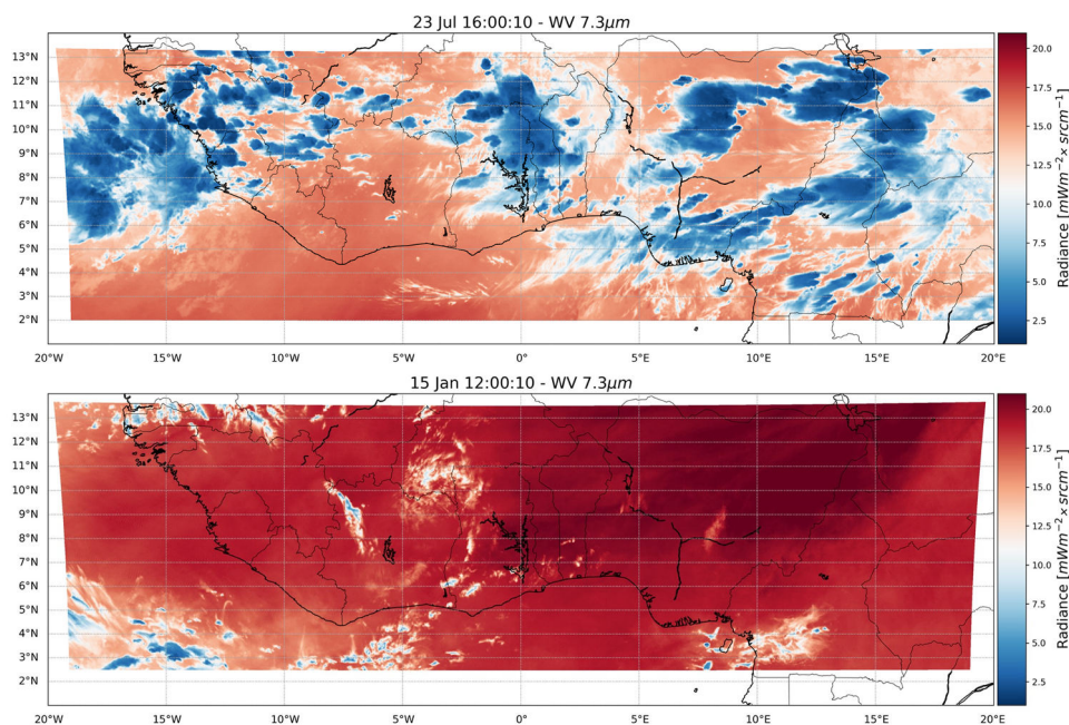
Figure 3.1: Illustration of the difference between rain (a) and dry (b) season as seen in 7.3 \mu\text{m} imagery: (a) Easterly moisture transport during boreal summer under the influence of midlevel jets. (b) Dry low-level wind blowing from Sahara desert slightly visible during dry season.
