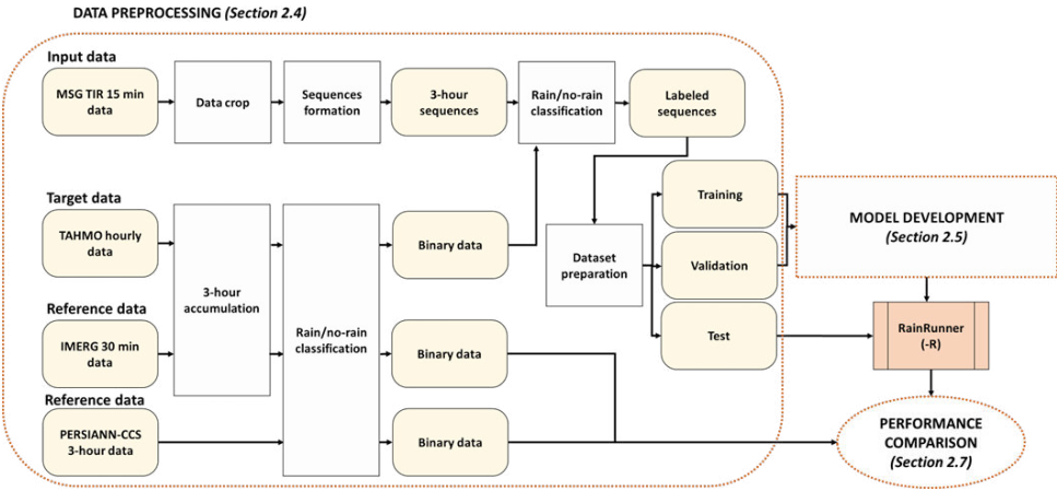
Figure 2.3: Overall flow diagram of the methodology followed in this study, from data preprocessing to performance comparison.
