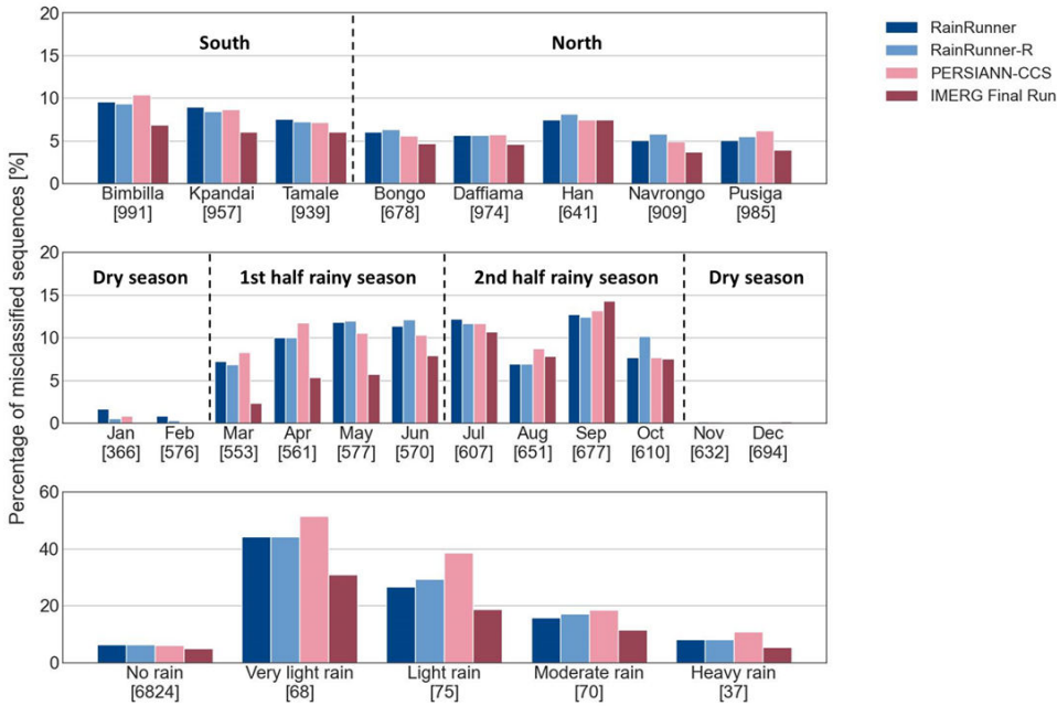
Figure 2.12: Misclassification analysis according to (top) station, (center) month, and (bottom) rainfall intensity. The numbers in brackets below the x-axis represent the number of sequences of each category in the test dataset.
