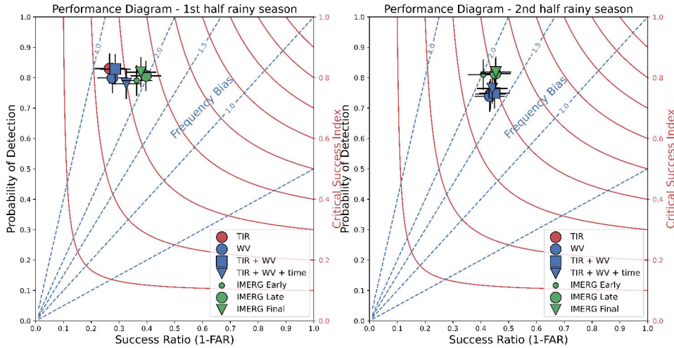
Figure 4.8: Performances of the four RainRunner models and IMERG Early, Late and Final runs on the Sudanian Savanna dataset, divided in the two halves of the rainy season.
