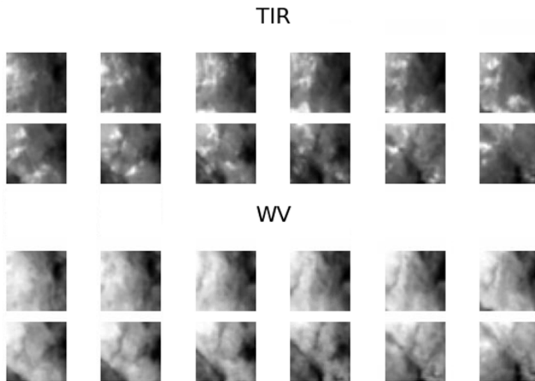
Figure 4.15: Example of a case when the addition of WV information corrected false alarms of the TIR-only model. Station TA00336 on the 20th of May 2019.
