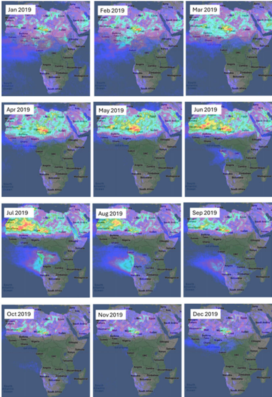
Figure 5.1: Monthly averages of the AER_{AI} product of the satellite Sentinel 5P, for 2019. The colour scale (ranging from dark blue to cyan, green, yellow, and red) represents aerosol presence, with green to red indicating a strong aerosol presence.
