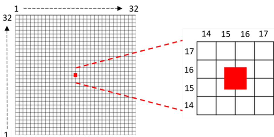
Figure 2.4: Center square in a 32 \times 32 pixels image. Here, pixels are numbered from bottom to top and from left to right.
