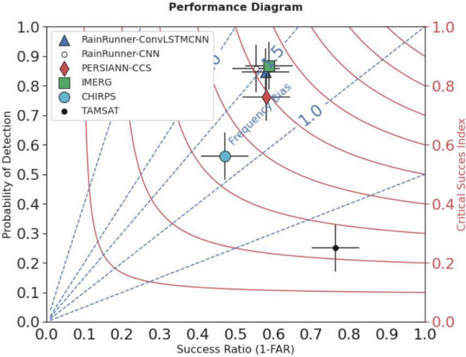
Figure 1: Performance diagram on the citizen science data.
