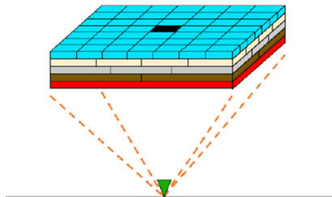
Figure 1.3: Concept of the link between multiple satellite information layers and one point rainfall measurement.
