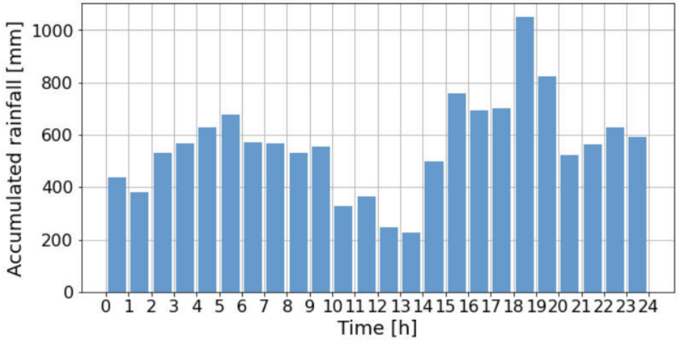
Figure 3: Total accumulated rainfall through the day, in 2019 and 2020 and at the 8 TAHMO stations.
