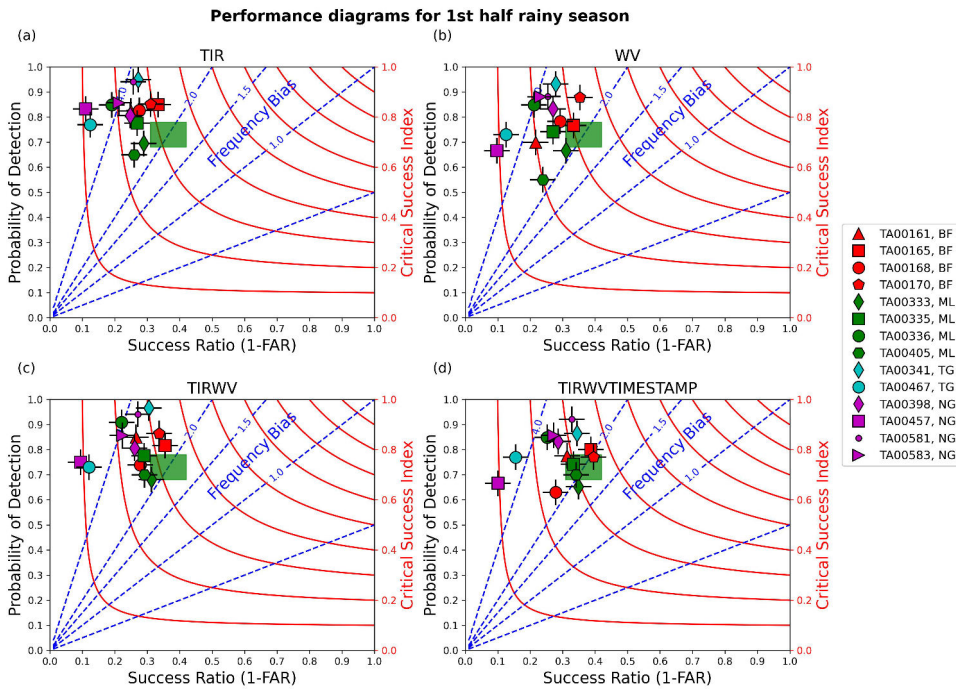
Figure 4.10: Performance diagrams during the first half of the rainy season. The green rectangle serves as reference and indicates the area comprised between the performances of the RainRunner models on the Northern Ghana stations. See Figure 3.7
