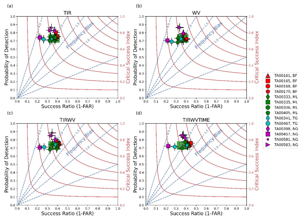
Figure 4.9: Performance diagrams of the RainRunner models on the Sudanian Savanna stations, for the entire study period (1/07/2018 to 31/12/2020). The green rectangle serves as reference and indicates the area comprised between the performances of the RainRunner models on the Northern Ghana stations. See Figure 3.7
