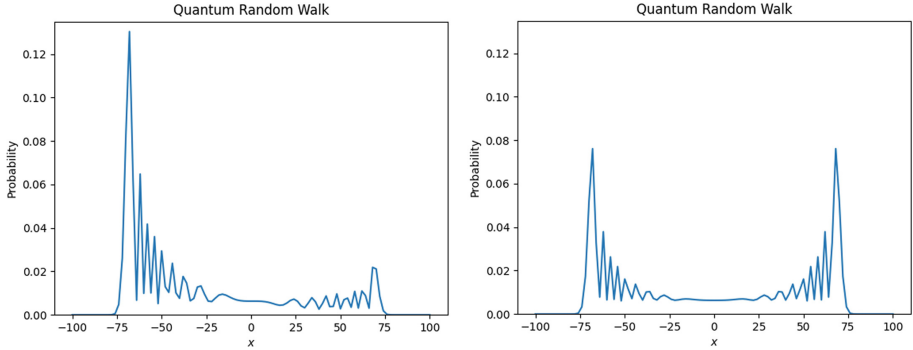
Fig. 8. Two Different Quantum Random Walks for the same Hadamard Coin Operator but Starting from a Different Initial Superposition. The Initial Superposition \frac{1}{2}\sqrt{2}|0\rangle \otimes (|0\rangle + |1\rangle) (Left) Versus the Initial Superposition \frac{1}{2}\sqrt{2}|0\rangle \otimes (|0\rangle + i|1\rangle) (right).
