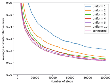
(a) Uniform Random Walk
