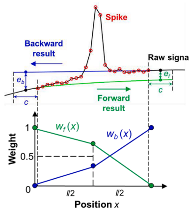
Fig. 7. Weighting functions.
