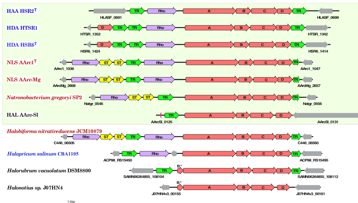
FIGURE 6 | Organization of gene clusters encoding polysulfide reductase (Psr) in haloarchaeal genomes. Arrows show the direction of transcription. Bar represents scale of 1000 bp and the genes are drawn to scale. Organisms with proven capability of lithotrophic sulfur-reducing growth using hydrogen as the electron donor are boxed. The members of orders Halobacteriales , Haloferales and Natrialbales are highlighted in blue, black and red, respectively. The genes associated with neither Psr reductase subunits (A-D, red) nor sulfur-transferases (ST, yellow), rhodanese-sulfurtransferase (Rho, violet) and transcriptional regulators (TR, green) are shown in gray colors.
