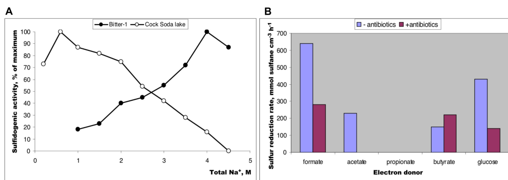
FIGURE 1 | Sulfur-reducing activity in anaerobic sediment slurry mix (1:1 with brines) from soda lakes in Kulunda Steppe (2011) incubated at 25° for 3–7 days. (A) Influence on salinity (as sodium carbonates) on potential sulfur reduction with formate as e -donor in sediments from moderately saline Cock Soda Lake and hypersaline Bitter-1 lake; (B) influence of antibiotics (streptomycin + kanamycin + vancomycin, 200 mg L -1 each) on potential sulfur reduction in sediment slurry from a mix sample prepared from 3 hypersaline soda lakes: Tanatar-1, Bitter-1, and trona crystallizer (Kulunda Steppe, Altai, Russia). The lakes are located in a close proximity and had have a similar brine characteristics (see Supplementary Table S1 ). The maximum activity was estimated as an average value from two parallel replicated samples. Total sulfane is a sum of free HS - and the sulfane atoms of polysulfides.
