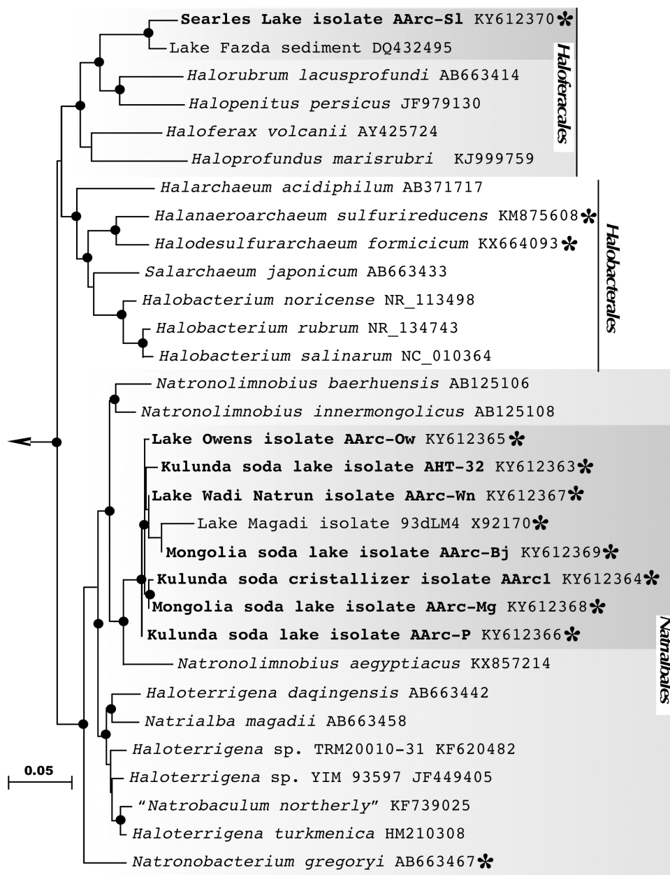
FIGURE 2 | 16S rRNA gene-based Maximum Likelihood phylogenetic tree showing the position of the sulfur-reducing natronoarchaea isolates (highlighted in bold) within the orders Haloferacales and Natrialbales . Members of the class Halobacteria , with experimentally confirmed ability for sulfur respiration, are highlighted by asterisks. Filled circles at the nodes indicate the bootstrap values > 70% (1000 bootstrap iterations). Methanohalophilus halophilus DSM 3094 T (GenBank accession no. FN870068) was used as an outgroup. Bar represents 0.05 substitutions per nucleotide position.
