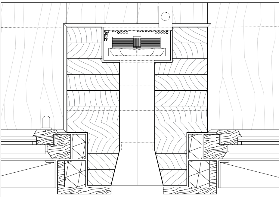
Breathing window detail
