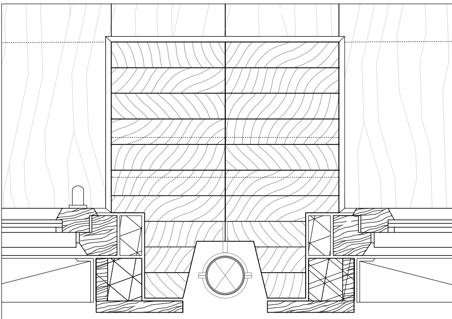
Rain gutter detail
