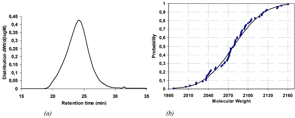
Figure 5: (a) Molecular weight distribution plot of an induction-heated bitumen at 110 °C (b) P-P plot of all the GPC samples, heated at four different temperatures, the original bitumen and the non heated samples
