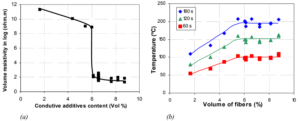
Figure 4: (a) Volume resistivity versus conductive particles content for mastic with sand-bitumen ratio 2.25
