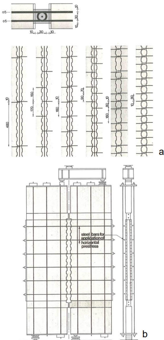
Figure 2.30: Internal reinforcement of the wall joint (a) and external steel bars for horizontal prestress (b) used by Hansen and Olesen (1976)
