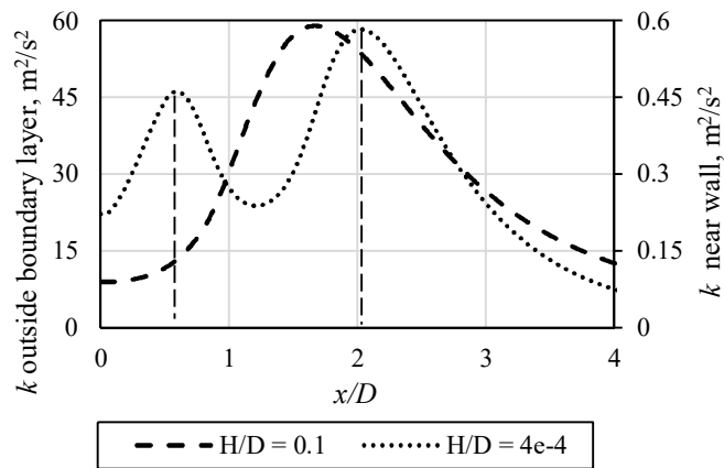
Fig. 5. Turbulence kinetic energy k distribution at line parallel to the heated surface, located outside boundary layer ( H/D = 0.1 ) and inside it ( H/D = 4\text{e-}4 ), \zeta-f model.
