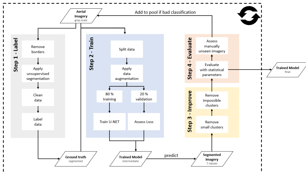
Figure 2. Flow chart of the processing chain from aerial imagery to trained model. All steps inside the dashed rectangle are applied in an iterative process.
