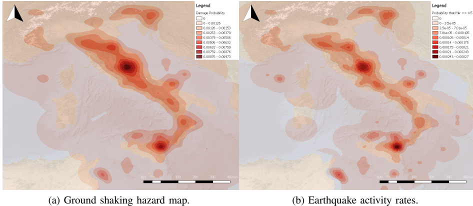
Fig. 1. An example of a ground-shaking hazard map (where the earthquake rates are converted in each cell of the grid, the probability that the intensity level equal to VI is exceeded during the next earthquake of M_w \geq 4.5 ) and earthquake activity rates (which are converted into probabilities that the next earthquake, which has the epicenter in a given cell of the grid, has a magnitude M_w \geq 4.5 ). Intuitively speaking (a) is a blurred version of (b).
