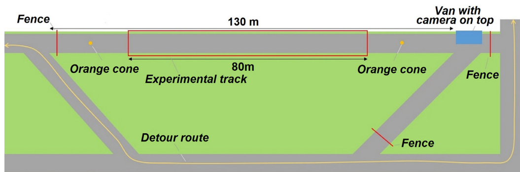
Fig. 2. Overview of experimental setup.
