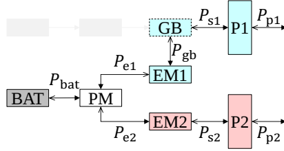
Fig. 6 Simplified models of the different powertrain architectures considered, including the power paths (indicated with lower-case subscripts), and powertrain components and energy sources (indicated with upper-case letters). Lines with two arrow heads indicate paths where the power can flow in both directions, with the positive direction shown by the filled arrowhead. Legend: “F” = fuel, “GT” = gas turbine, “GB” = gearbox, “P” = propulsor, “BAT” = batteries, “EM” = electrical machine (i.e. electromotor or generator), “PM” = power management and distribution system.
