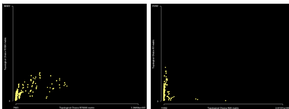
Figure 1. Two different scatterplots showing the correlation between the angular analyses with a high and a low metrical radius. The scatterplot to the left is from a vital neighbourhood where the scatterplot to the right is from a mono-functional problem neighbourhood.
