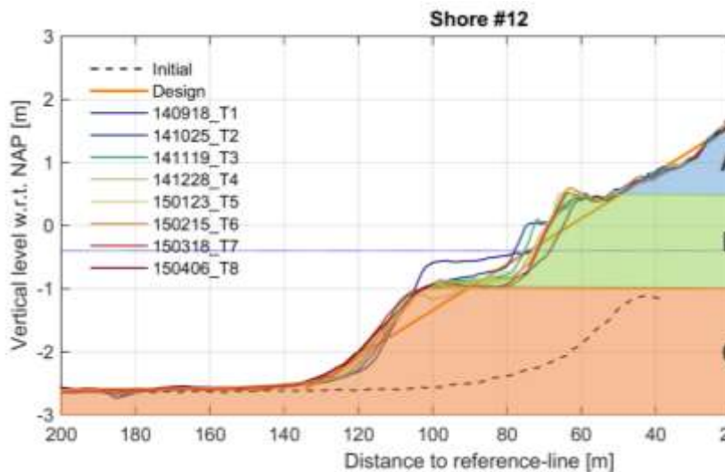
Figure 4-20 Cross-shore sections used in the volume analyses of the foreshore
