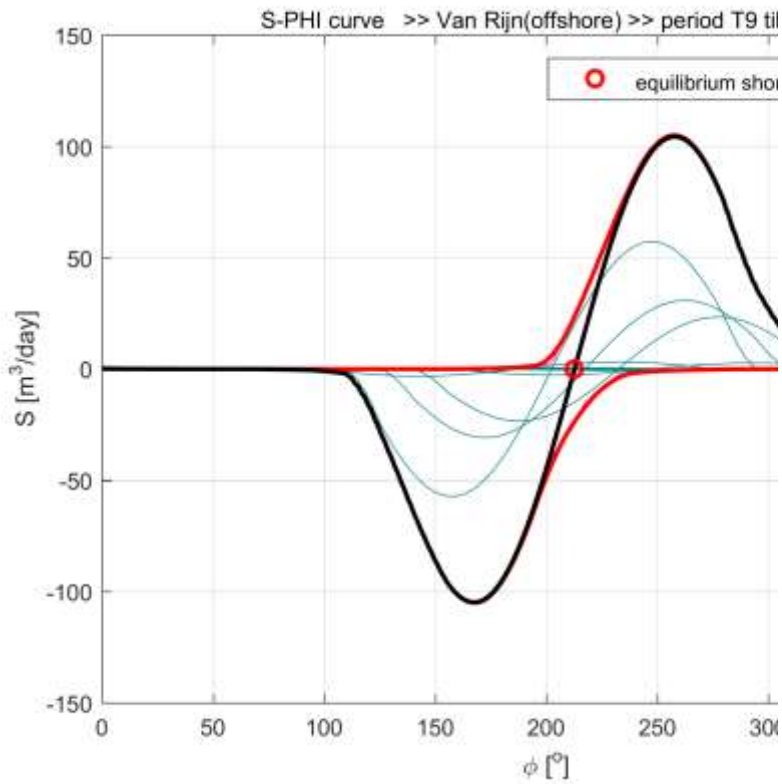
Figure 0-50 S-Phi curve with Van Rijn (2002) formulation for specific period (see title in figure)
