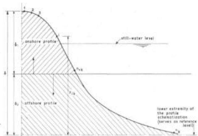
Figure 2-12 Left: Two-line theory schematization according to (Bakker, 1968)
