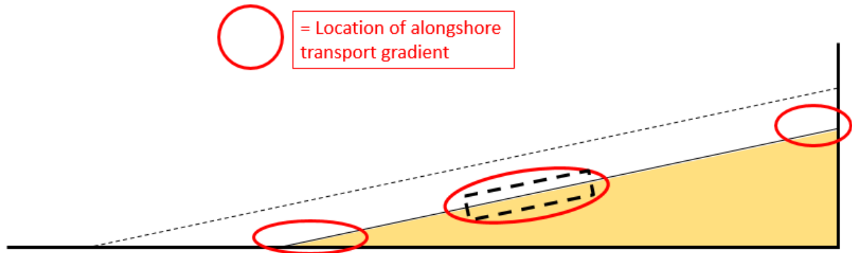
Figure 5-21 Locations of alongshore transport gradients on the foreshore of the Houtribdijk
