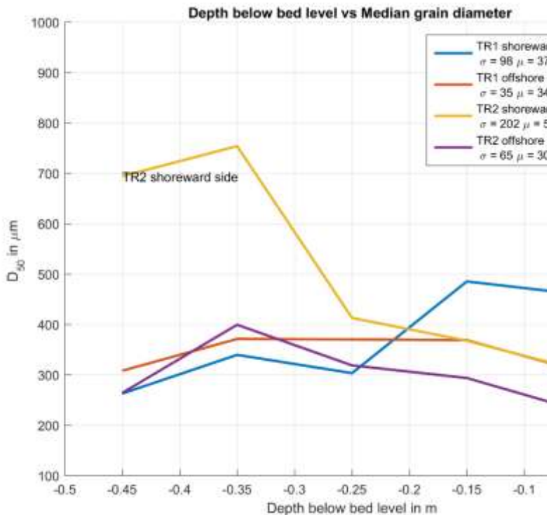
Figure 4-48 Measurements of median grain-size taken below bed level. At two transects (TR 1 and TR 2) sediment core samples are taken at the shoreward and the offshore side of the horizontal plateau. The standard deviation and average are displayed in the legend.
