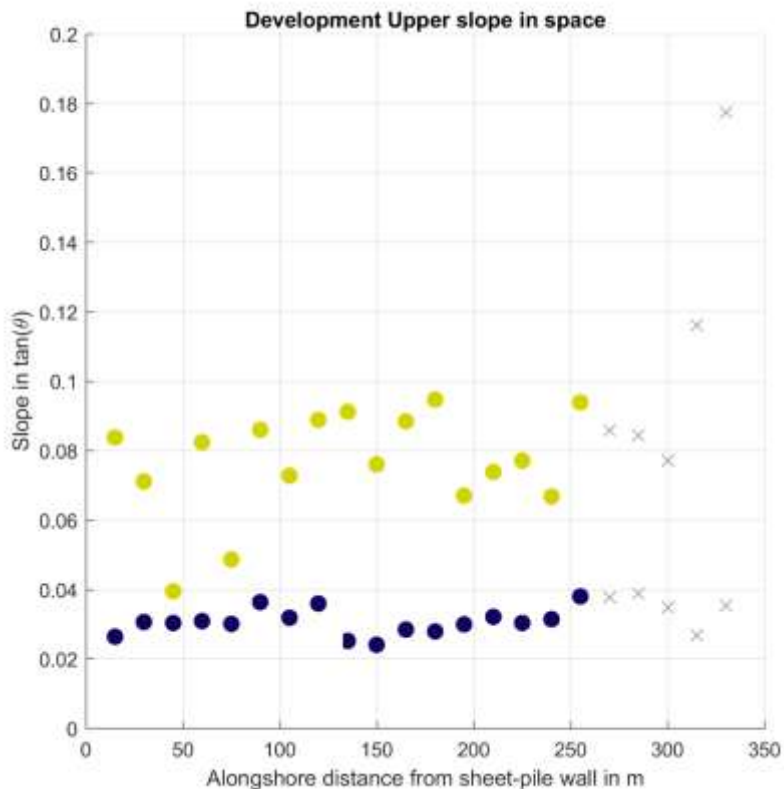
Figure 4-15 Spatial development of upper slope for all cross-shore profile rows. The sheet-pile wall is located at x=0 .
