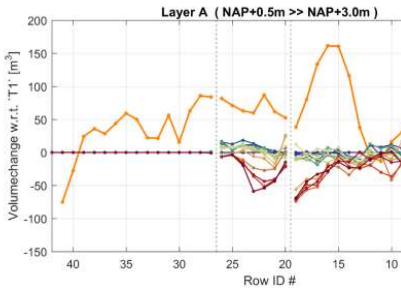
Figure 4-23 Alongshore volume changes in cross-shore layer A
