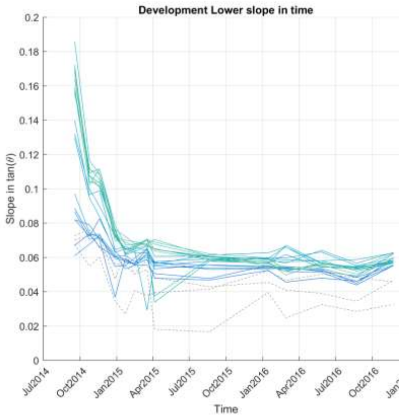
Figure 4-12 Temporal development of lower slope for all cross-shore profile rows. Shore # 4 is located at the sheet-pile wall
