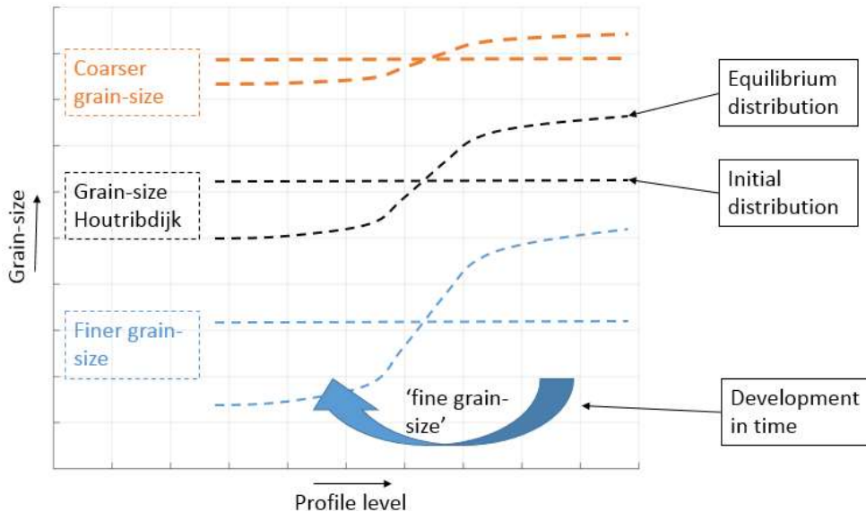
Figure 6-10 Conceptual representation of the effect of coarser/finer initial grain-size on the lower and upper slope angles.
