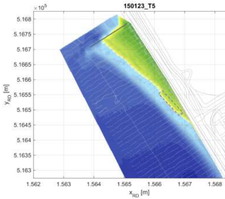
Figure 0-15 Measured bathymetry from T5 at 23/01/2015
