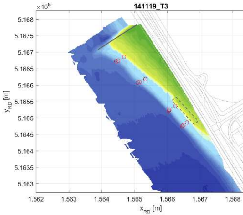
Figure 3-5 Locations of sediment samples, red circles, at the third measurement campaign
