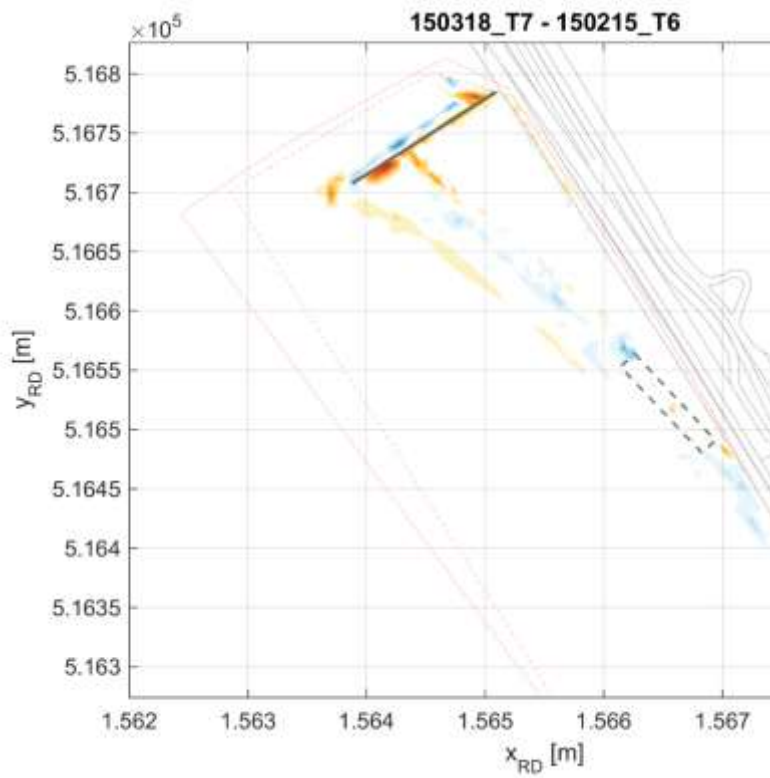
Figure 0-30 Measured difference in bathymetry in the period of T7 and T6
