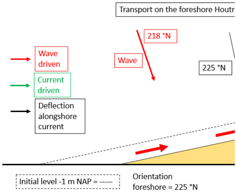
Figure 6-3 Conceptual model behaviour foreshore Houtribdijk
