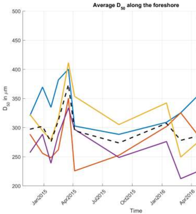
Figure 4-45 Temporal development of median grain-size ( D_{50} ) for all transects and the average on the foreshore
