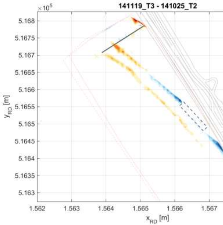
Figure 0-26 Measured difference in bathymetry in the period of T3 and T2
