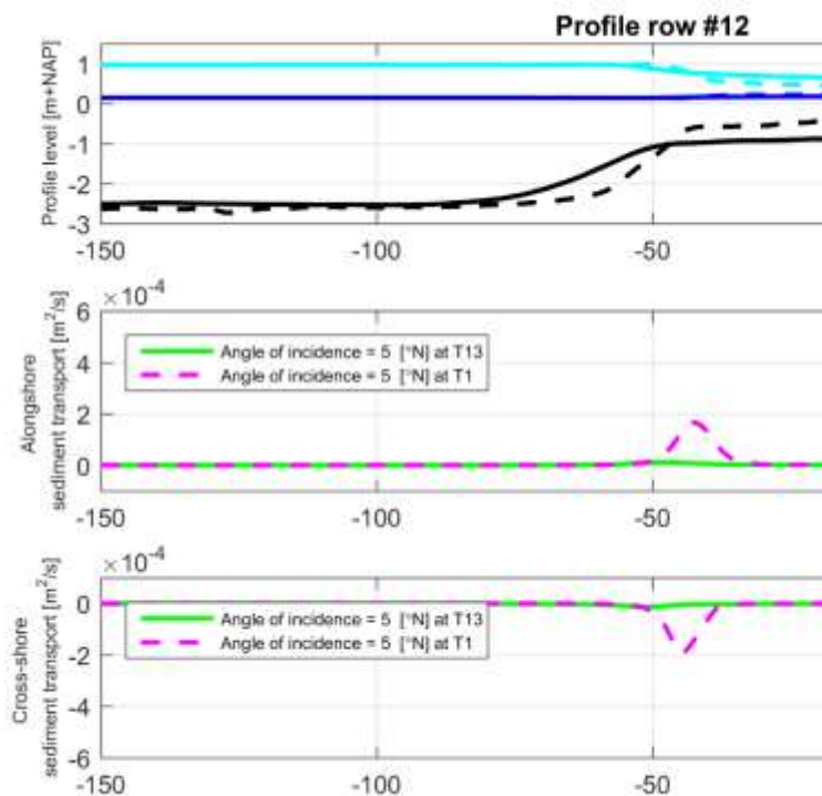
Figure 5-26 XBeach model results of alongshore and cross-shore transports for storm condition with H_s = 1.07 m and h = 0.15 m and wave incidence = 5. For the initial profile at T1 and profile at T13.
