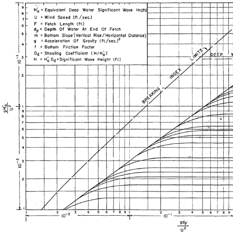
Figure 2-3 Generation of waves by wind over a bottom of constant level for unlimited wind duration. (source: (Bretschneider, 1964))
