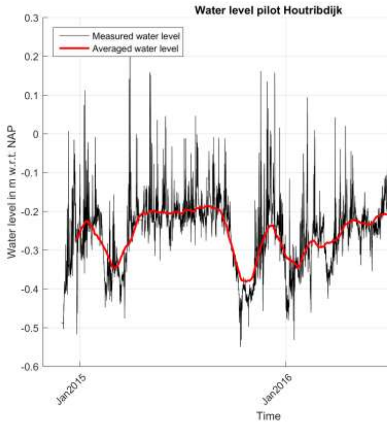
Figure 4-53 Measured water level during the monitoring of the Pilot Houtribdijk. The red coloured line represents the averaged water level.
