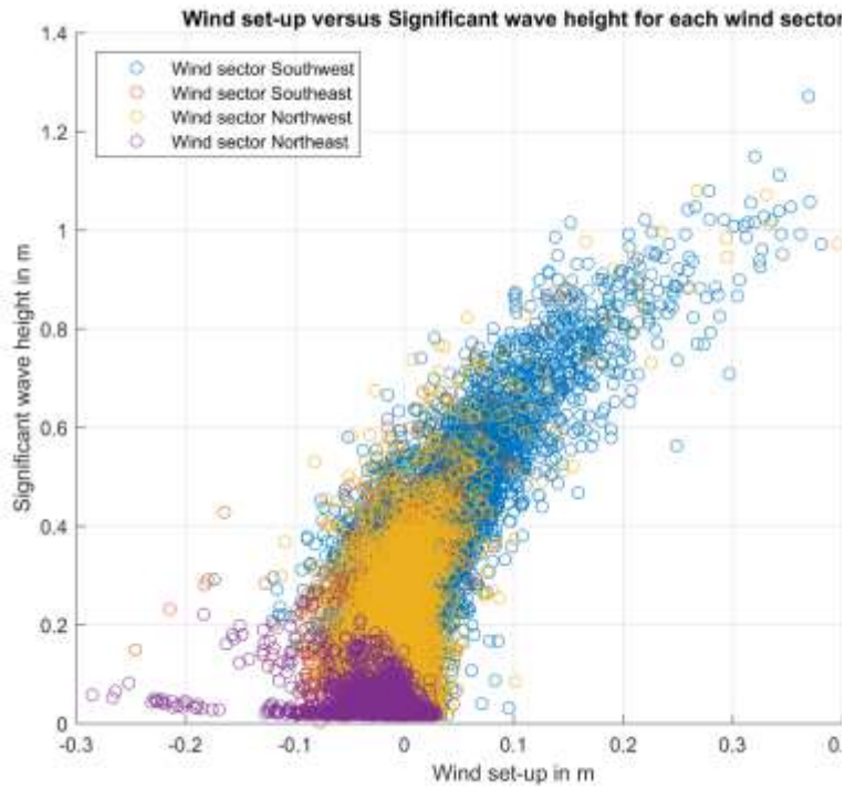
Figure 4-55 Relationship wind set-up and significant wave height. The marker colours indicate the wind direction during measurements.
