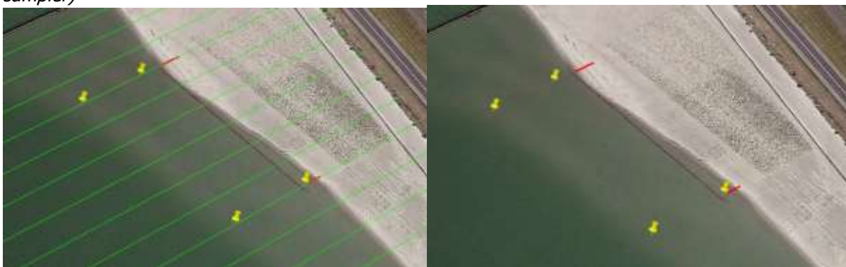
Figuur 2 Location measured depth rows and sediment sampling locations (red line are the sampling locations taken with a Van Veen grabber, yellow markers are the locations of sediment core samples with piston sampler)
