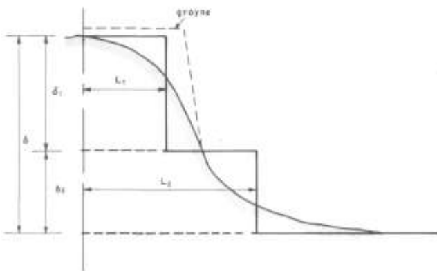
Figure 2-12 Left: Two-line theory schematization according to (Bakker, 1968)
