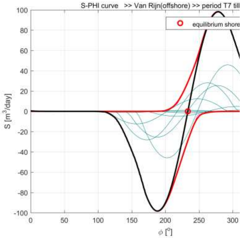
Figure 0-46 S-Phi curve with Van Rijn (2002) formulation for specific period (see title in figure)
