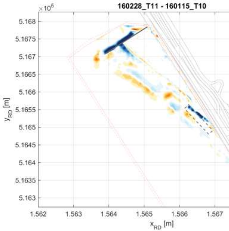
Figure 0-34 Measured difference in bathymetry in the period of T11 and T10
