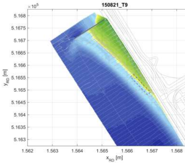
Figure 0-19 Measured bathymetry from T9 at 21/08/2015
