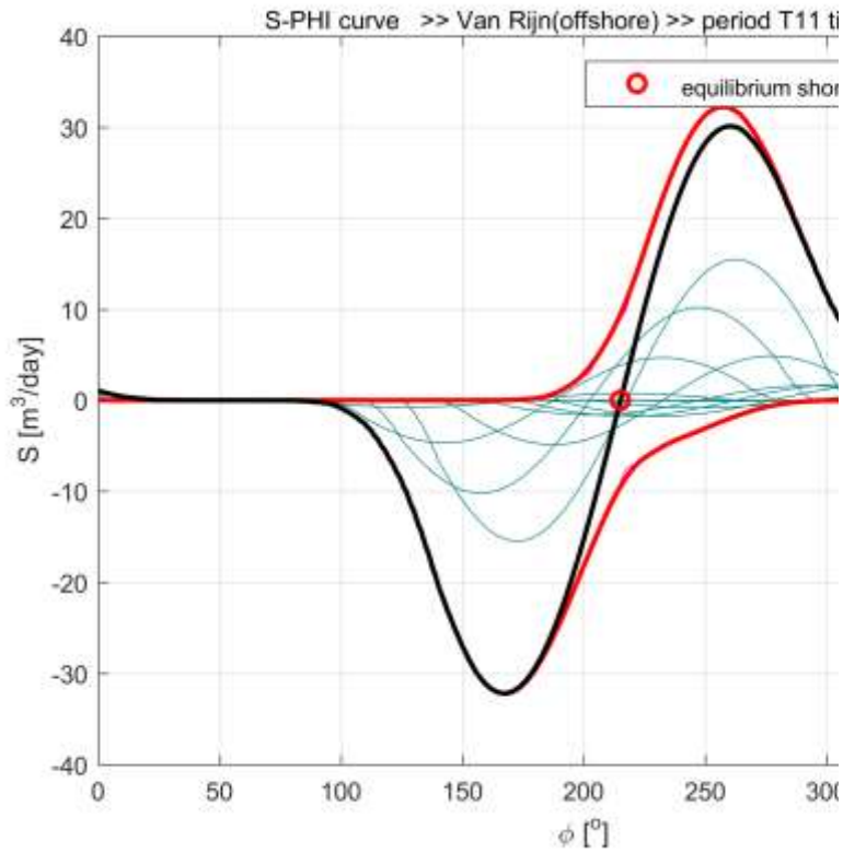
Figure 0-54 S-Phi curve with Van Rijn (2002) formulation for specific period (see title in figure)
