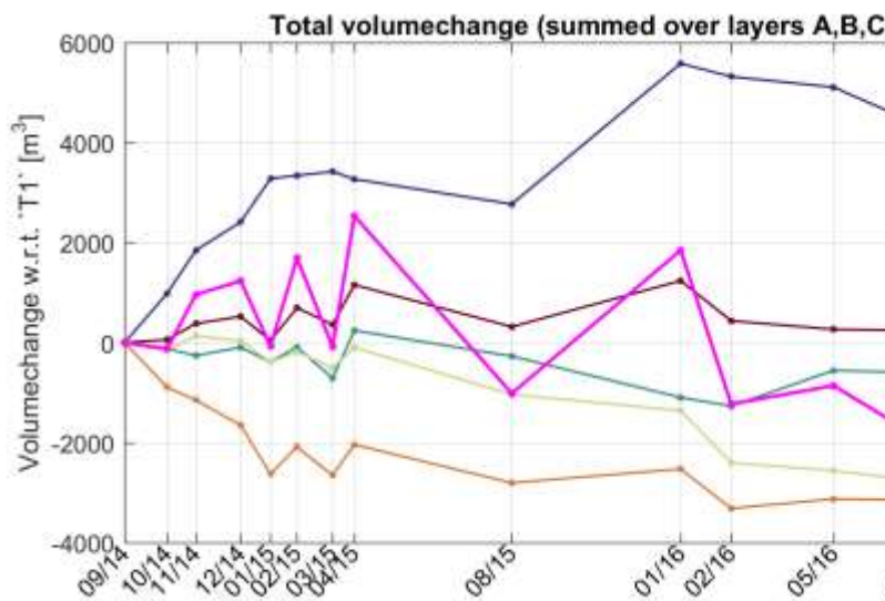
Figure 4-27 Total volume change for alongshore sections 1, 2, 3, 4 and 5 in time summed for all three cross-shore layers.
