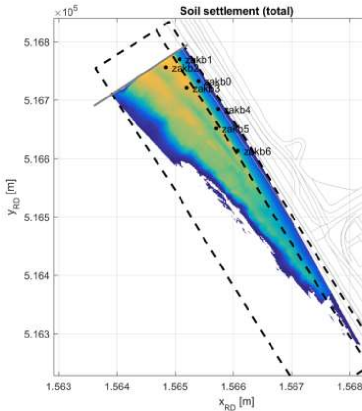
Figure 4-30 Estimated settlement of the initial bed after the construction of the foreshore at T1 (18/9/2014). (source: (Arcadis, 2016))
