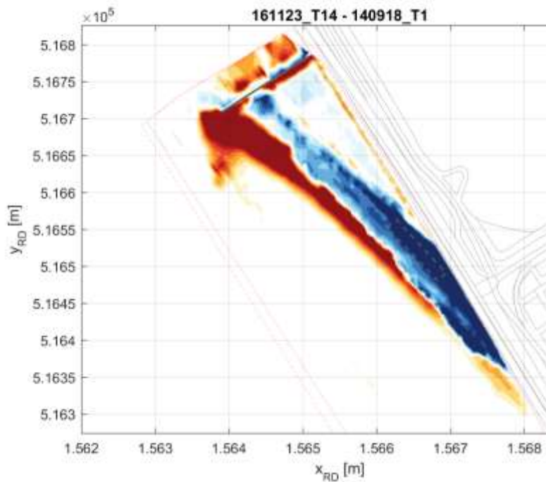
Figure 4-3 Difference in bathymetry on the foreshore between measurement campaign T1 (18/09/2014) and T14 (23/11/2016), blue colours represent erosion and red colours represent sedimentation
