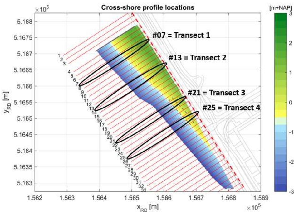
Figure 3-4 Overview of the four representative transects for the bathymetric and sediment analyses (source: (EcoShape, 2016c))
