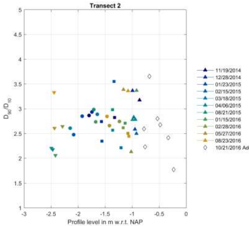
Figure 4-42 Measurements sorting of grain-size D_{90}/D_{10} plotted versus the profile level along transect 2. The colours represent the measurement campaigns and the markers indicate the original level rows the sediment sample was taken. \blacktriangle is NAP -0.500 m, \blacksquare is -1,0 m NAP, \bullet is -1,5 m NAP, \blacktriangledown is -2,0 m NAP, \diamond are additional measurements
