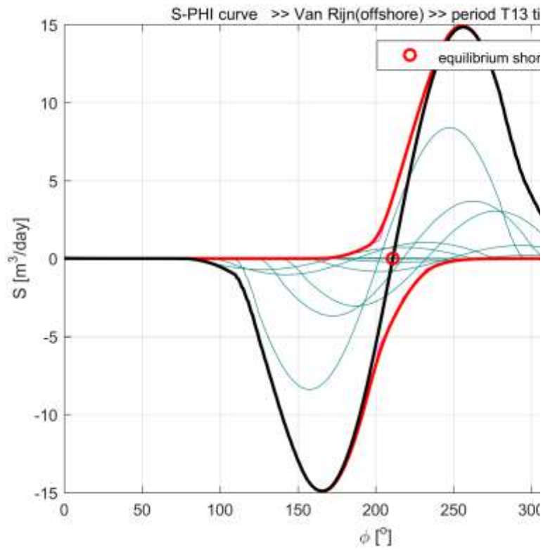
Figure 0-58 S-Phi curve with Van Rijn (2002) formulation for specific period (see title in figure)
