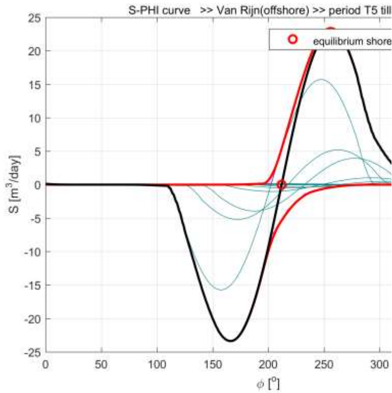
Figure 0-42 S-Phi curve with Van Rijn (2002) formulation for specific period (see title in figure)
