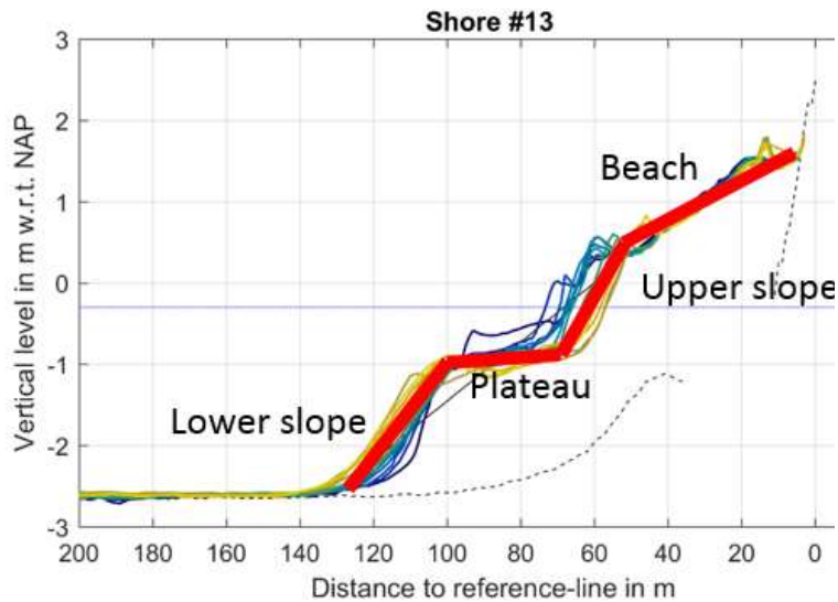
Figure 4-9 Schematization of cross-shore profile shape
