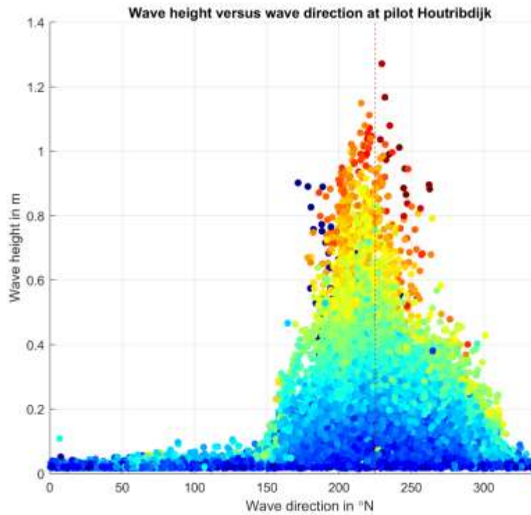
Figure 4-50 Significant wave height plotted against wave direction. The marker colours indicate the corresponding wind speed.
