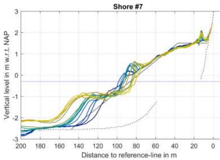
Figure 4-5 Cross-shore profile measurements from T1 (18/09/2014) till T14 (23/11/2016) of profile row 7 of the foreshore. Black dotted line represents the initial profile along the Houtribdijk.
