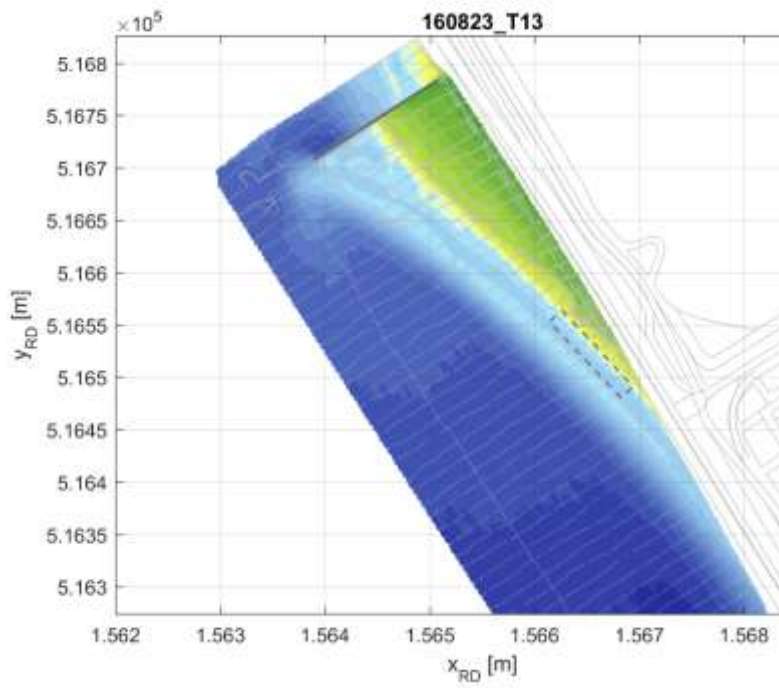
Figure 0-23 Measured bathymetry from T13 at 23/08/2016
