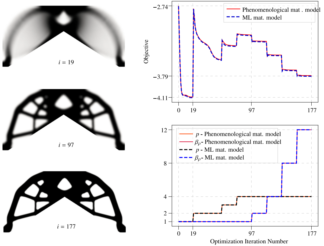
Fig. D.14. Convergence history for portal frame TO problem. Visualized designs correspond to those corresponding to TO using ML model at iterations where critical continuation parameter updates occur.
