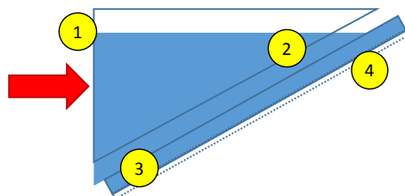
Fig. 7. IG WFE contributors, originating from the prism and wafer. #1 and #2 are surface WFE of the prism. #3 is the wafer thickness variation. #4 is the grating WFE. To obtain the total infrared WFE, all parameters have to be multiplied by the index of refraction of the Si material ( n=3.4 ), and parameters #1, #2 and #3 have to be multiplied by a factor of 2 (double pass). The geometric angle of incidence must also be taken into account.
