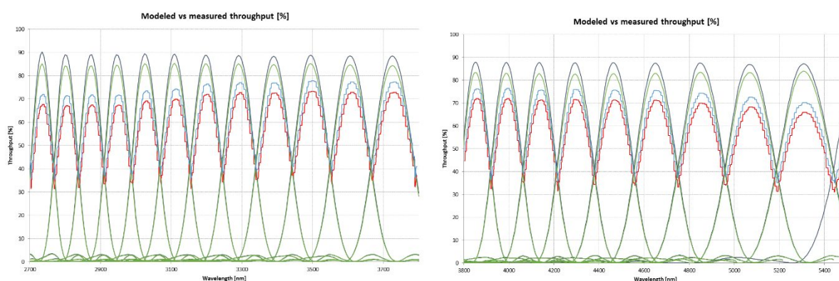
Fig. 3. Throughput of the IG is shown for the 2.7\mu\text{m} – 3.8\mu\text{m} – 5.5\mu\text{m} wavelength range. Going from the curve with the highest peaks towards the curve with the lowest peaks, line #1 shows the modelled diffraction efficiency of the IG, #2 shows the modelled diffraction efficiency + AR coating, #3 shows the calibrated measurement data without the effect of the defected areas and #4 depicts the calibrated measurement data.
