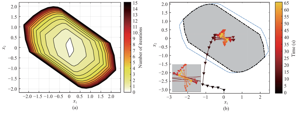
Fig. 4. Visualization of MPDT GRPI set and evolution of the difference system. (a) shows the computation process of Algorithm 2, where the white set denotes the initial set O_0 and the darkest set denotes O([\tau, T]^T) . In (b), evolution of state trajectory is demonstrated in 2D view, where the inner shadowed set is O([\tau, T]^T) and the outer blue dashed line denotes the \mathcal{G}([\tau, T]^T) . A zoom-in display is presented in the bottom of (b) to have a detailed view of the state trajectory.
