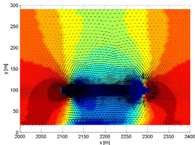
Figure 4.48: Water-level depression and velocity field around an eccentrically sailing ship (from red to blue: increasing water level depression). Image by TU Delft – Ports and Waterways is licenced under CC BY-NC-SA 4.0.
