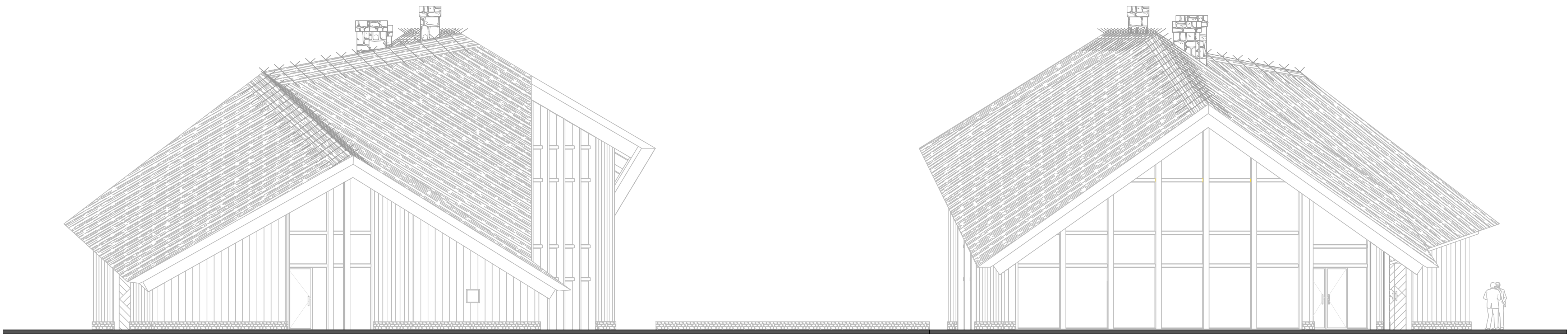
WEST ELEVATION | 1:100
