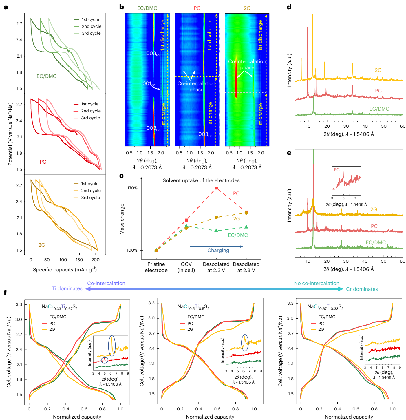
Fig. 5 | Co-intercalation in other layered sulfides. a , Voltage profiles of P3- \text{Na}_x\text{V}_2\text{S}_5 in EC/DMC, PC and 2G electrolytes at 0.1 C showing different behaviours. Three-electrode measurements in Swagelok-type cells were used to minimize the influence of counter-electrode polarization. b , Results from operando XRD of P3- \text{Na}_x\text{V}_2\text{S}_5 electrodes cycled in EC/DMC, PC and 2G at 0.125 C. Similar to P2- \text{Na}_x\text{TiS}_2 , a large lattice expansion indicative of solvent intercalation occurs with PC and 2G. c , Relative mass of P3- \text{Na}_x\text{V}_2\text{S}_5 electrodes in the pristine state (before cell assembly), at OCV (electrodes are wetted), and after desodiation to 2.3 V and 2.8 V versus \text{Na}^+/\text{Na} in the different electrolytes. The large mass increase for PC
