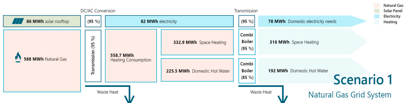
Figure 8. Energy consumption diagram of Scenario 1: natural gas grid system, utilizing light renovation (graphic illustrated by author).
