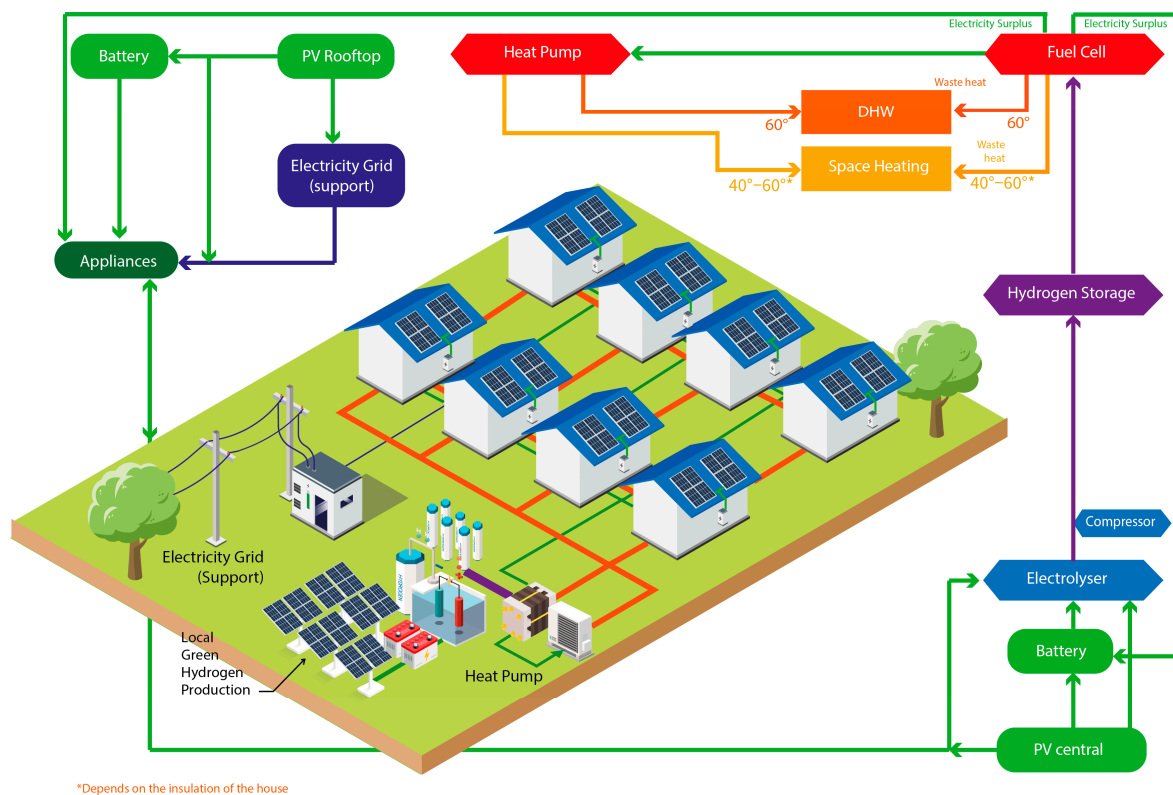
Figure 17. An illustration of energy system design for Scenario 6: hydrogen hybrid heat pump system (Author illustration).
