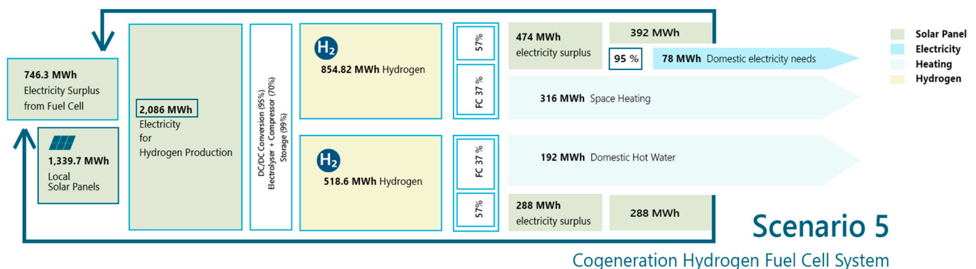
Figure 16. Energy consumption diagram of Scenario 5: cogeneration hydrogen fuel cell system, utilizing light renovation.
