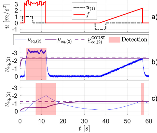
Fig. 4. (a) Input of lead vehicle and cyber-attack. (b), (c) Second element of EOI with its lower threshold. Vertical axes are inverted to highlight the estimation capability of the SMO. (b) Fast parameters; (c) Slow parameters.
