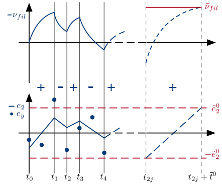
Fig. 1. Example healthy EOI response - t_0 \leq t \leq t_4 ; Worst-case EOI response for the peak threshold design - t_{2j} \leq t \leq t_{2j} + \bar{t}^0 . Both with corresponding e_2 behaviour.
