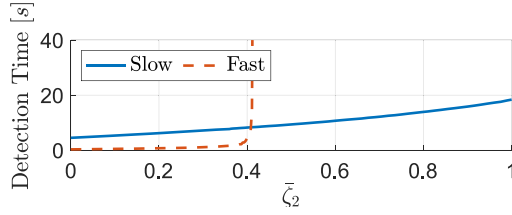
Fig. 3. Detection time of a step attack of 2.8 m/s 2 for different measurement noise bounds \zeta_2 . \zeta_1 = 1 is kept constant.
