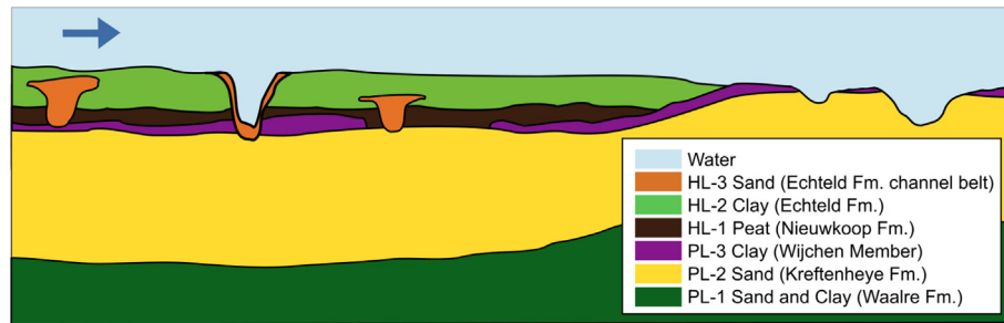
Fig. 1. Conceptual longitudinal subsurface lithological longitudinal section of a river bed, with typical distances of 10 to 20 m in depth and 10 to 20 km in length. Arrow indicates flow direction. In colour the lithological formations (Fm.) and members are indicated. Scour holes form in layers or patches composed of sandy material with lower erodibility compared to the surrounding resistant clay or peat layers.
