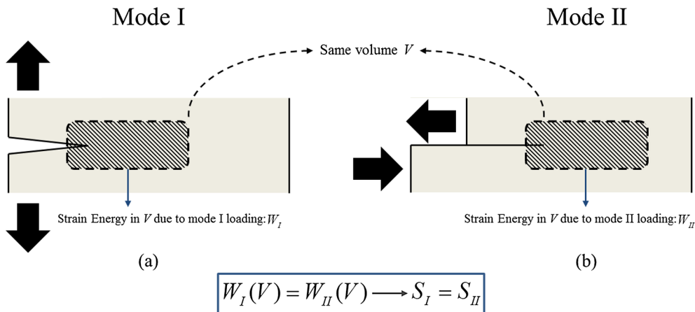
Fig. 2. (a) Cracked body under pure mode I; (b) Cracked body under pure mode II. Both cracked bodies are from the same material. The strain energy density ( S ) that causes fracture is the same for both loading modes (reproduced from [13]).
