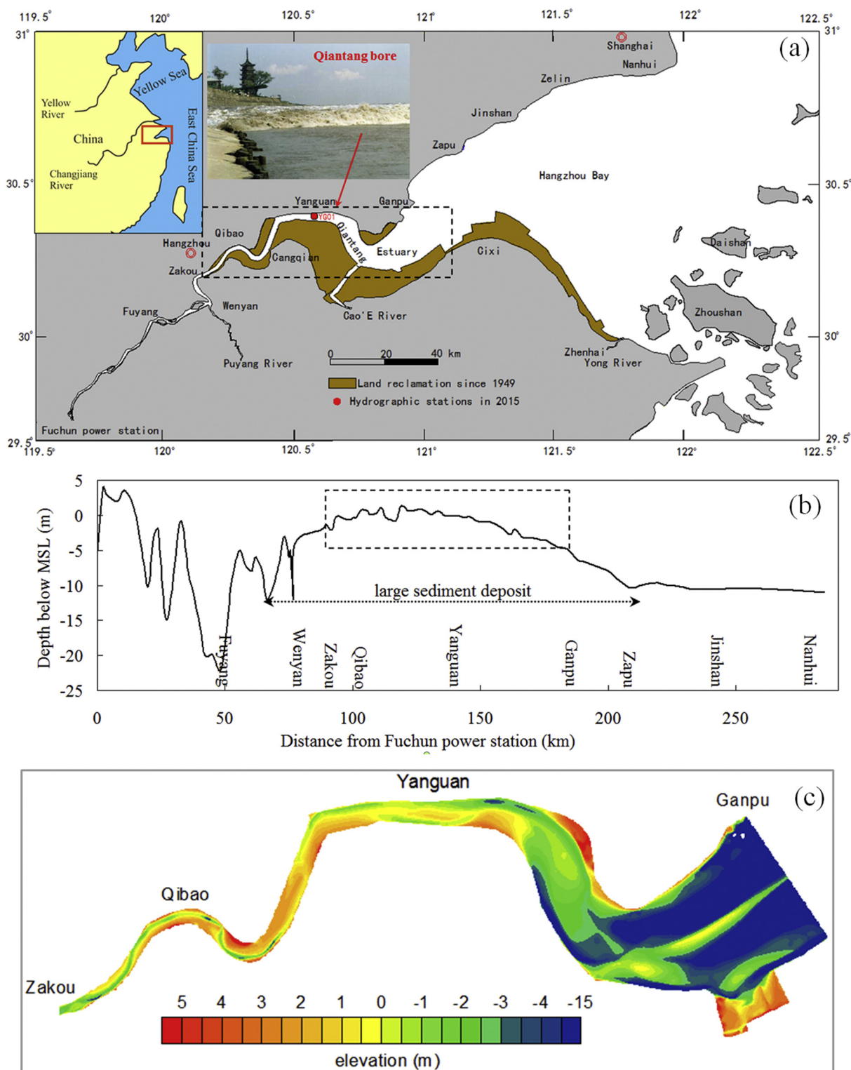
Fig. 1. (a) Location of the Qiantang Estuary, in which YG01 denotes the hydrographic observation station in October 2015. (b) The lateral-averaged longitudinal bathymetry along the estuary measured in 2014. (c) Bathymetry of the middle estuary measured in April 2015. Panels a and b were modified from Xie et al. (2017a). The bed elevations in panels b and c are with respect to the Chinese National Vertical Datum of 1985. The dashed box in panels a and b denotes the middle reach of the estuary, as shown in panel c.
