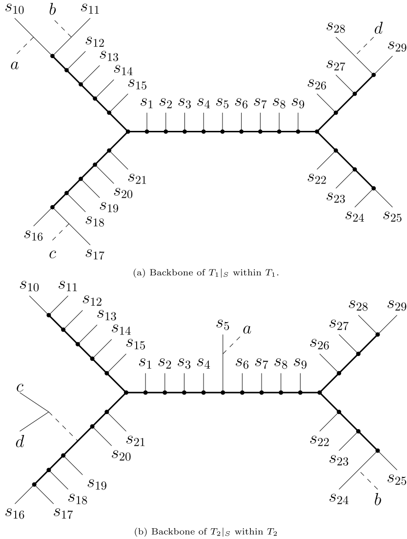
Fig. 2. Example illustration of the backbone of T_1|_S = T_1|_S = T_2|_S within T_1 and T_2 , where S = \{s_1, \dots, s_{29}\} . Edges and vertices of the backbone are in bold. Observe that T_1|_S has the chain s_1, \dots, s_9 , but (T_1, T_2) do not have a common chain of length greater than 4, as the leaf s_5 has a sibling a in T_2 .
