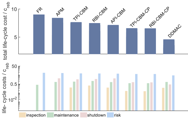
Fig. 5. Comparison of DDMAC life-cycle policies with different baseline policies. Total life-cycle cost and life-cycle costs due to inspection, maintenance, shutdown, and risk (95% confidence intervals are lower than \pm 1\% ). The best optimized baseline is 42% worse than the DDMAC policy.
