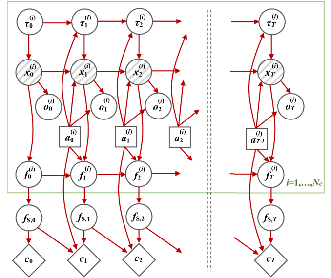
Fig. 4. Dynamic Bayesian network of multi-component deteriorating system in time.
