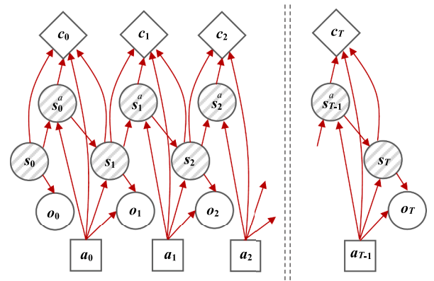
Fig. 1. POMDP diagram in time, including intermediate states occurring after actions and before environment transitions.
