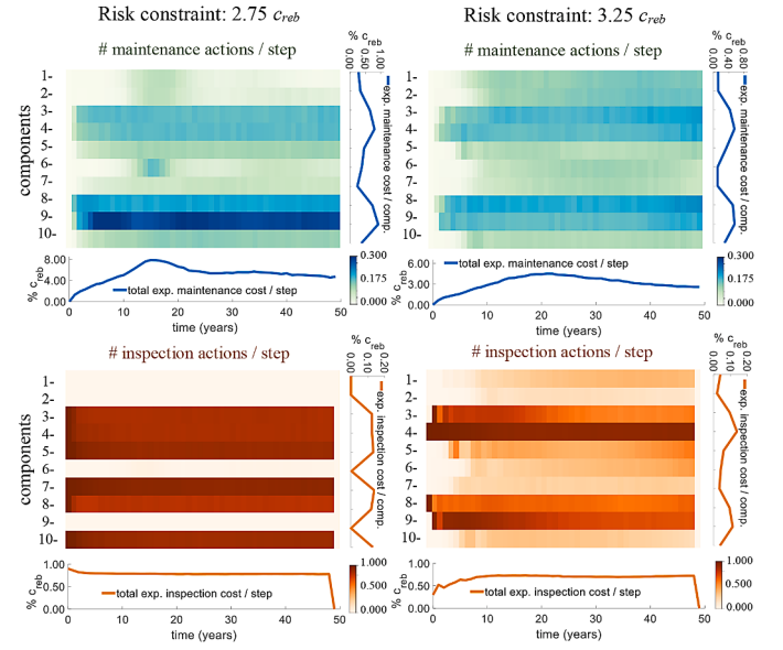
Fig. 9. Components maintenance and inspection frequency per step and respective mean costs for risk constraints of 2.75 and 3.25\ c_{reb} (95% confidence intervals are lower than \pm 0.5\% ).
