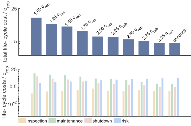
Fig. 7. Comparison of DDMAC life-cycle policies for different life-cycle risk constraints from 1\ c_{reb} to infinity. Total life-cycle cost and life-cycle costs due to inspection, maintenance, shutdown, and risk (95% confidence intervals are lower than \pm 0.5\% ).
