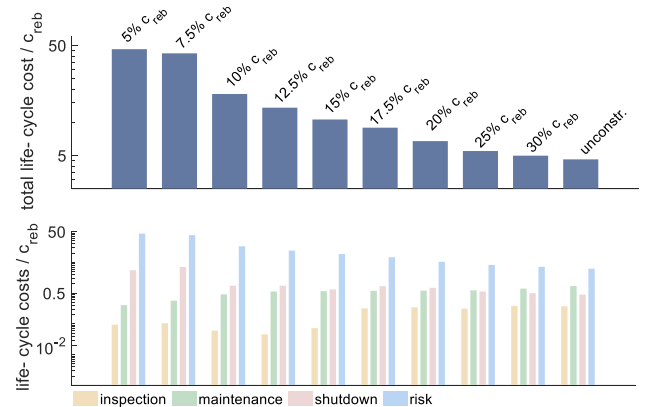
Fig. 6. Comparison of DDMAC life-cycle policies for different 5-year constraints from 5% c_{reb} to infinity. Total life-cycle cost and life-cycle costs due to inspection, maintenance, shutdown, and risk (95% confidence intervals are lower than \pm 0.5\% ).
