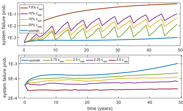
Fig. 12. System mean failure probabilities based on DDMAC life-cycle policies for different (a) 5-year budget constraints and (b) life-cycle risk constraints (95% confidence intervals are lower than \pm 0.5\% ).
