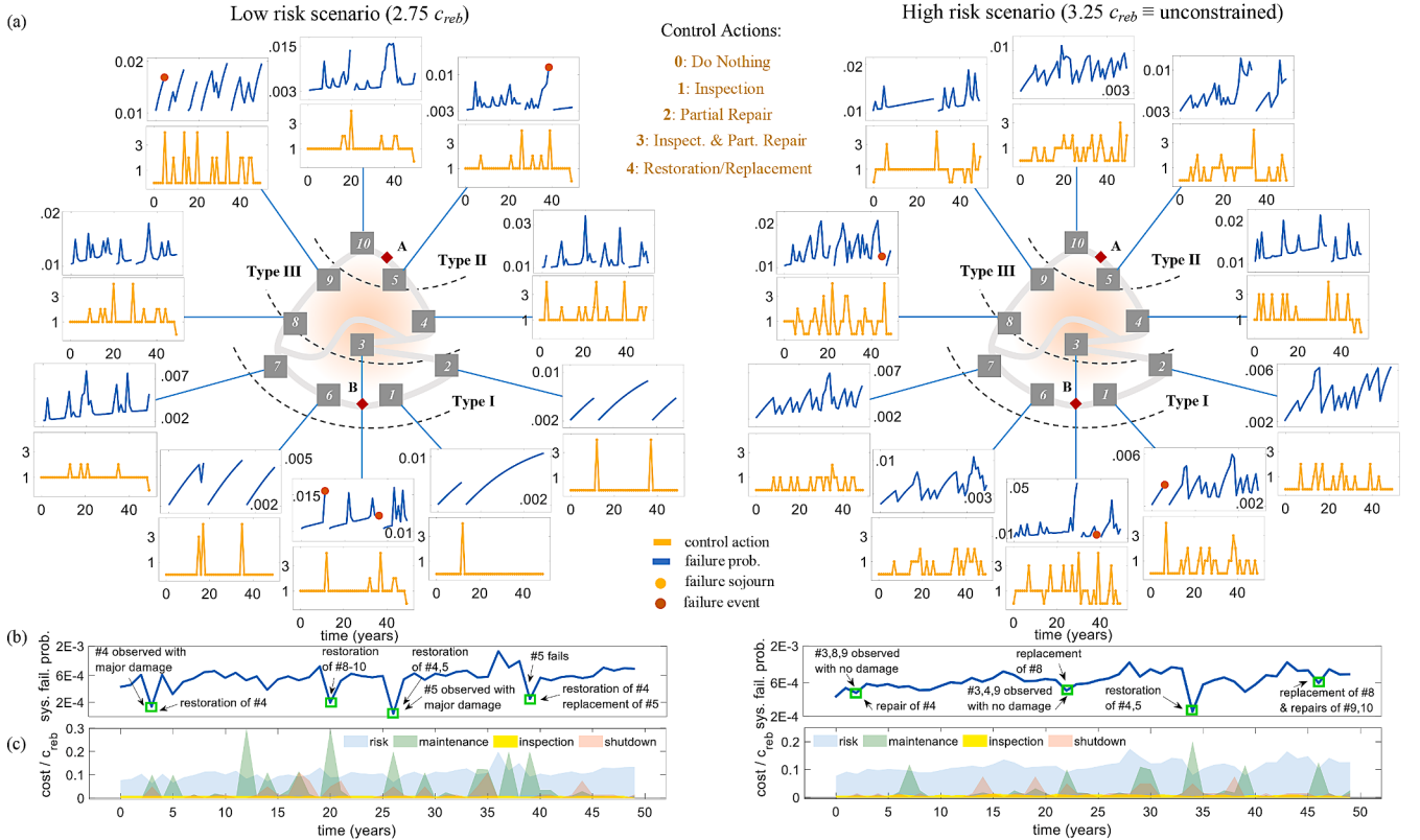
Fig. 11. Life-cycle realization of the learned DDMAC policy for 2.75 c_{reb} and 3.25 c_{reb} life-cycle risk constraints. (a) Component failure probabilities and actions; (b) System failure probability with selected interventions; (c) Costs of inspection and maintenance actions, scheduled shutdowns, and risks.
