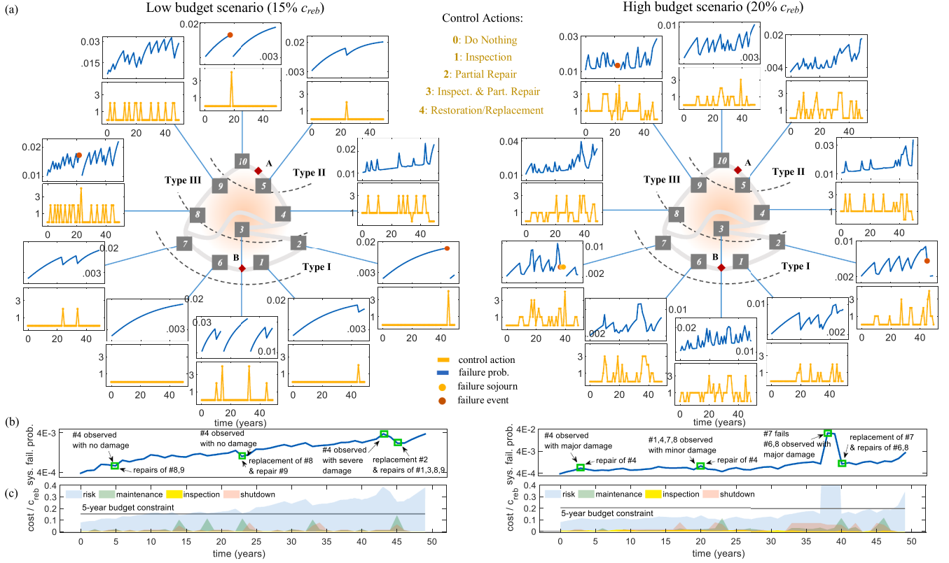
Fig. 10. Life-cycle realization of the DDMAC policy for 15% c_{reb} and 20% c_{reb} 5-year budget constraints. (a) Component failure probabilities and actions; (b) System failure with selected interventions; (c) Costs of inspection and maintenance actions, scheduled shutdowns, and risks.
