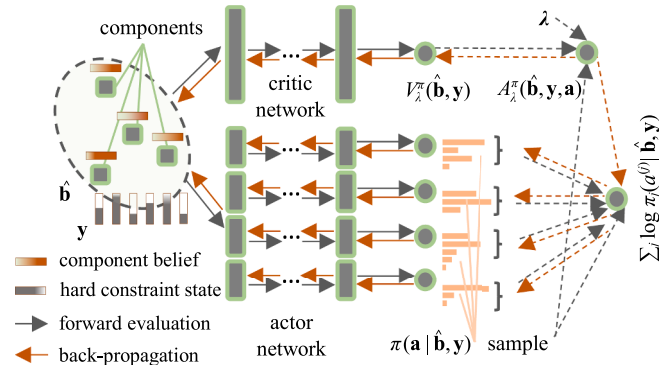
Fig. 2. Constrained Deep Decentralized Multi-agent Actor Critic (DDMAC) architecture.
