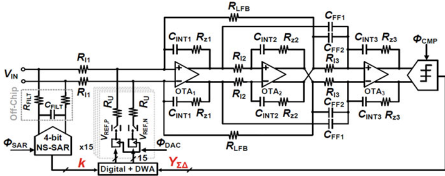
Fig. 21 Simplified schematic of the proposed CT zoom ADC
