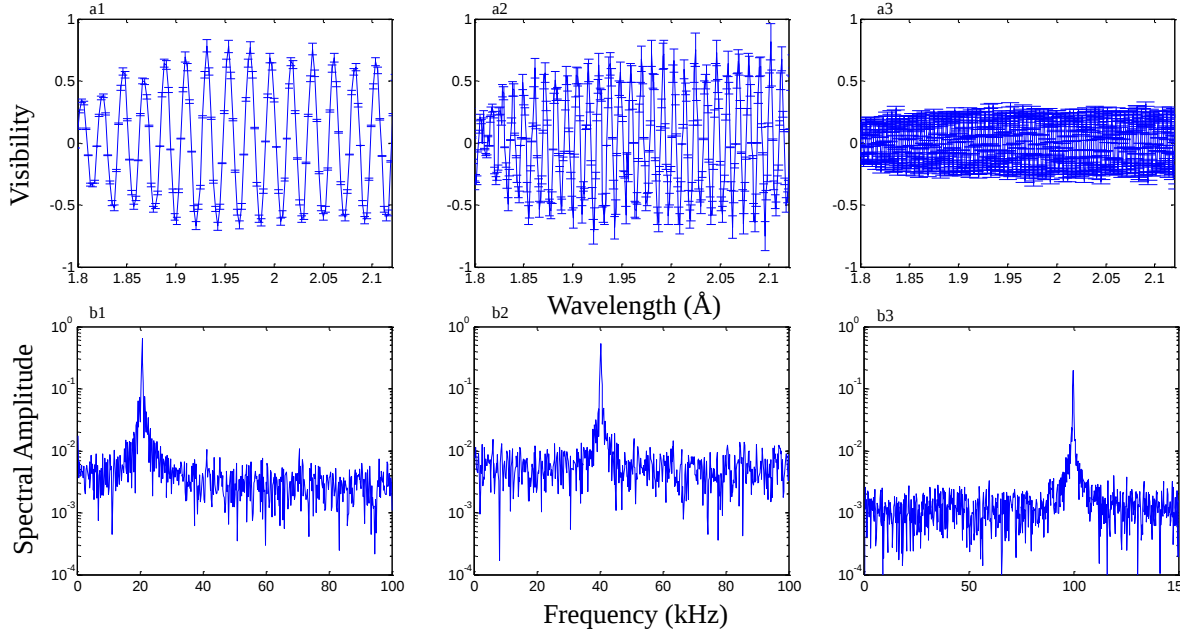
Figure 7. MIEZE signal (a1-a3) and FFT (b1-b3) for 20 kHz, (a1-b1), 40 kHz (a2-b2) and 100 kHz (a3-b3). Note the declining amplitude as the frequency increases. This is due to the fact that the detector thickness limits the time resolution. Furthermore errors due to timing inaccuracies (i.e. triggering of the function generators), become prominent as the frequency increases.
