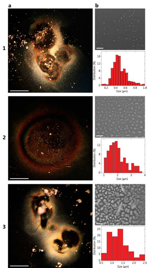
Figure 4. Morphology of MOF derivatives. Optical images (a), SEM micrographs and diameter distribution (b) for corresponding derivatives obtained from compounds 1 , 2 , and 3 . Scale bars, 50 \mu\text{m} (a); 10 \mu\text{m} for 1 and 2 (b), and 5 \mu\text{m} for 3 (b).
