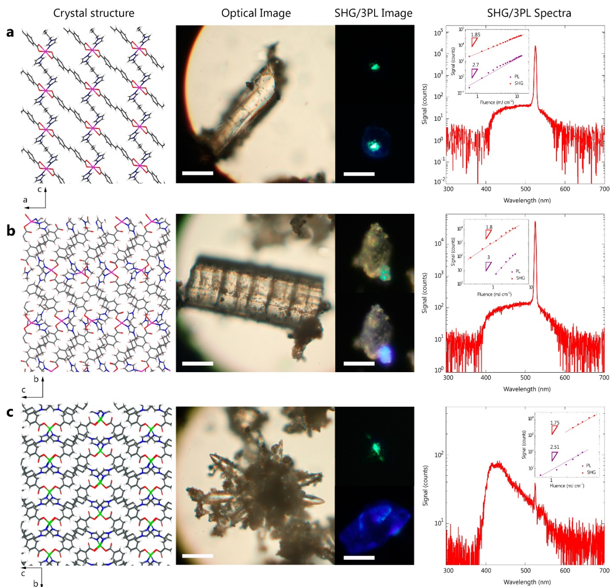
Figure 2. Characterization of initial MOFs. Crystal structure, optical image, SHG/3PL images as well as spectra of SHG/3PL with corresponding quadratic and cubic slope (inset) for compound 1 (a), 2 (b), and 3 (c). Scale bars, 10 \mu\text{m} and 5 \mu\text{m} for optical and SHG/3PL images, respectively.
