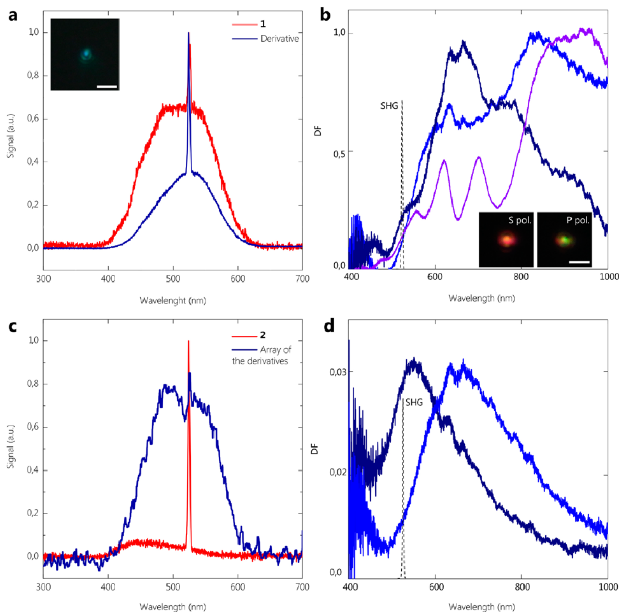
Figure 6. Optical properties of MOF derivatives. SHG and 3PL spectra from the derivatives of 1 (a) and 2 (c) normalized by maxima. Inset: optical image of SHG-3PL signal from single derivative. Scale bar, 2 \mu\text{m} . (b,d) Corresponding spectra of scattering of s polarized white light in dark-field geometry on single derivatives with diameter ranging from 500 to 800 nm. The number of resonances (maxima of the curves) corresponds to intrinsic Mie-type modes generated inside the derivatives [15] . Inset: optical image of derivative irradiated by s and p polarized light. Scale bar, 2 \mu\text{m} .
