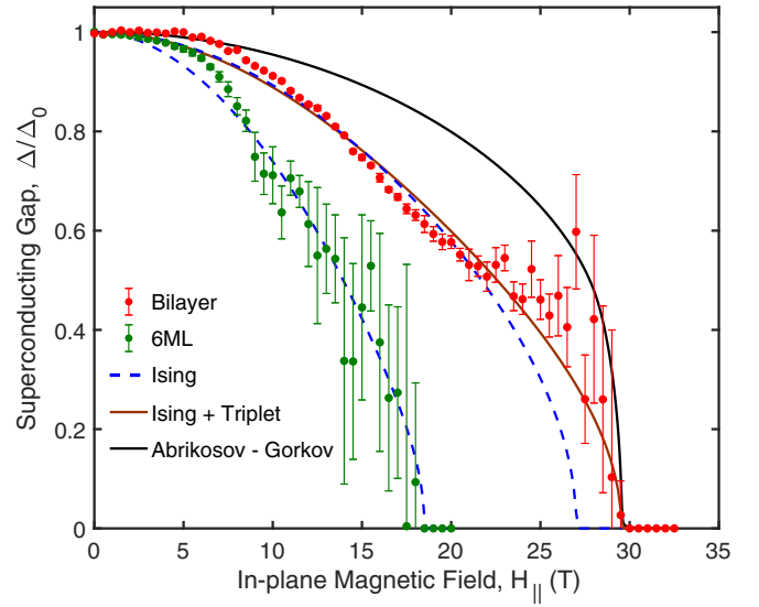
FIG. 4. Normalized superconducting gap as a function of the in-plane magnetic field \Delta(H_{\parallel}) obtained from the fits of the quasiparticle density of states in Fig. 3. The error bars were obtained following the procedure described in Supplemental Material Sec. I A. The blue dashed curves are a fit of experimental data using the Ising theory alone. Here, E_{SO} = 14.45T_{cs} (with T_{cs} = 2.6 K) for the bilayer sample and E_{SO} = 2.21T_{cs} (with T_{cs} = 5.4 K) for the six-monolayer (6ML) sample. In brown is the Ising theory with an equal-spin triplet component of the order parameter as described in the text. Here, E_{SO} = 9.62T_{cs} and T_{ct} = 0.05T_{cs} , with T_{cs} = 2.6 K. Finally, the solid black curve is calculated using the Ising theory with strong disorder (equivalent to the Abrikosov-Gor’kov theory). In all cases, the critical field is constrained to be the experimental one.
