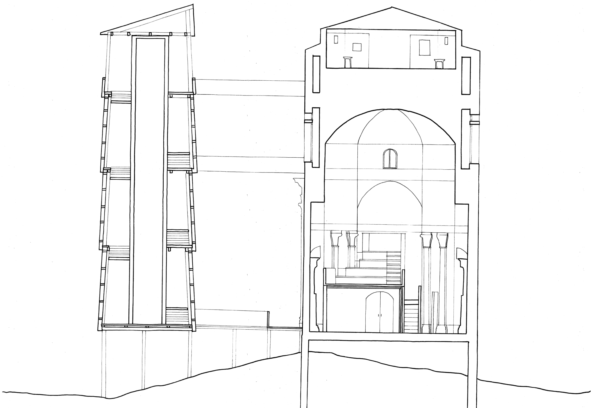
Section 1:100
