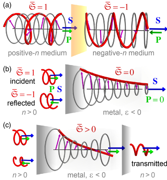
FIG. 1. Schematic picture of the helicity ( \tilde{\mathcal{G}} = \omega \mathcal{G}/W ), canonical momentum, and spin, when a circularly polarized plane wave (a) propagates through an interface between positive-index ( \epsilon > 0, \mu > 0 ) and negative-index ( \epsilon < 0, \mu < 0 ) media, (b) is reflected from a metallic semispace ( \epsilon < 0, \mu > 0 ), and (c) is partially transmitted through a metal film. The red curves and magenta arrows indicate the spatial distribution of the instantaneous electric field \text{Re}(\mathbf{E}e^{-i\omega t}) , whereas the gray circles show the time evolution of the field at fixed positions.
