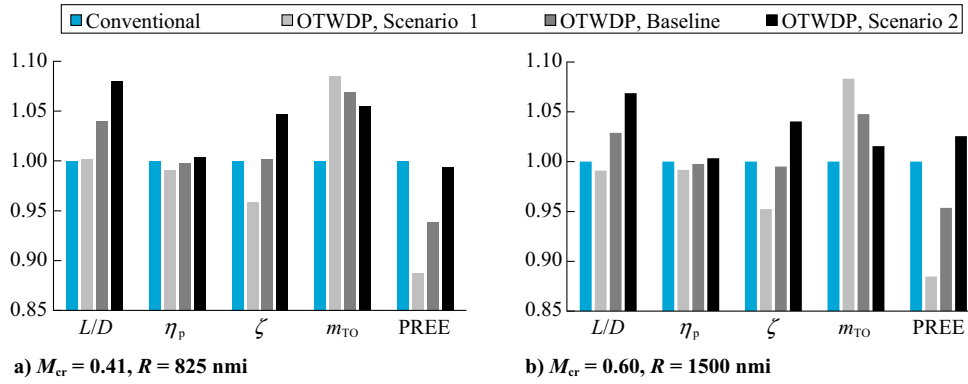
Fig. 11 Effect of aerodynamic-model assumptions on aircraft performance parameters. All values are normalized with the corresponding reference-aircraft values.
