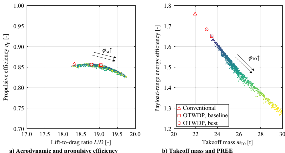
Fig. 13 Top-level aircraft performance metrics for various combinations of shaft-power ratio \phi as obtained from the DOE. Darker colors indicate higher PREE values. M_{cr} = 0.41 , and R = 825 n miles.
