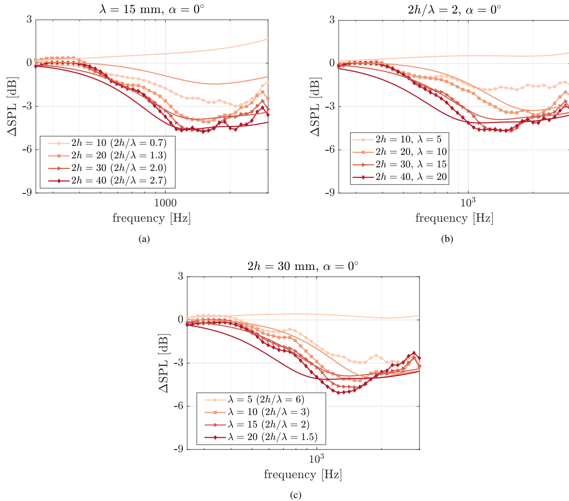
Fig. 8 Predicted (solid line) and measured (line with markers) noise reduction from serrated trailing edges mounted on a symmetric benchmark airfoil NACA 63 3 -018 at zero angle of attack (dimensions in millimeters). (a) shows the predicted noise reduction variation with changing serration height (same serration wavelength, \lambda = 15 mm). (b) shows the predicted noise reduction variation with changing serration size (same serration aspect ratio, 2h/\lambda = 2 ). (c) shows the predicted noise reduction variation with changing serration wavelength (same serration height, 2h = 30 mm).
