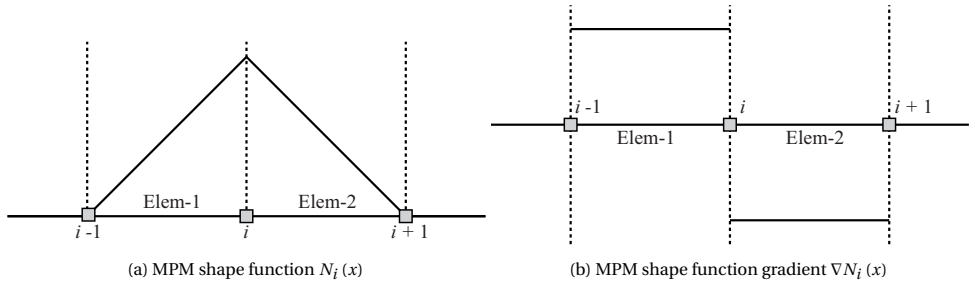
Figure 2.3: Standard MPM shape function N_i(x) and its gradient \nabla N_i(x) in 1D case
