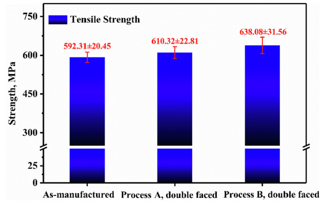
Fig. 12. Effect of shot peening on tensile properties of FMLs.
