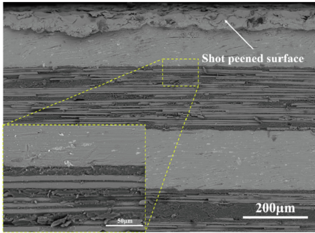
Fig. 7. The SEM morphology of shot peened FMLs.
