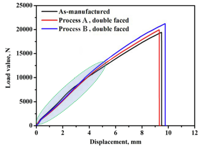
Fig. 9. Tensile load-displacement curves of FMLs before and after shot peening.
