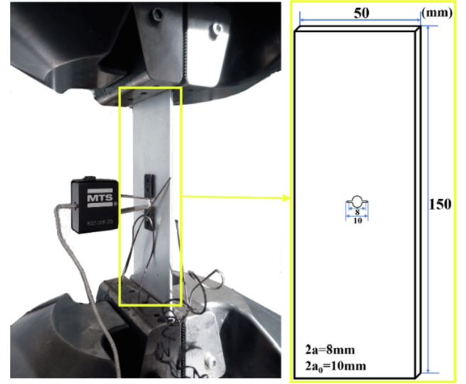
Fig. 5. The FCG test of FMLs.
