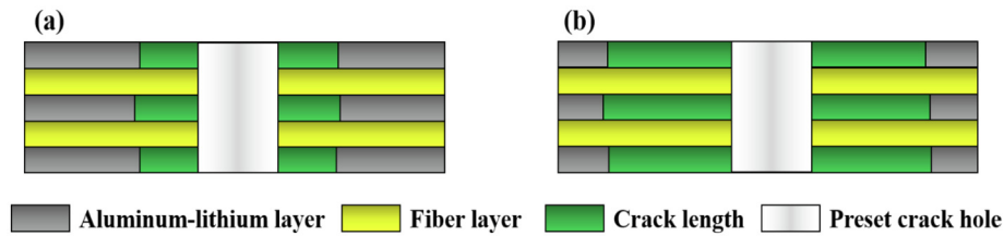
Fig. 15. crack length in internal and external layers of FMLs shot peened by process B: (a) crack reached about 13.3 mm; crack reached about 26.6 mm.
