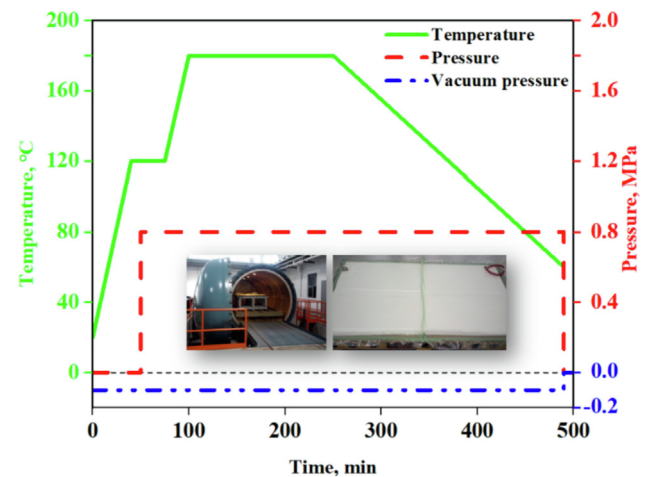
Fig. 2. The curing process of the FMLs in autoclave.
