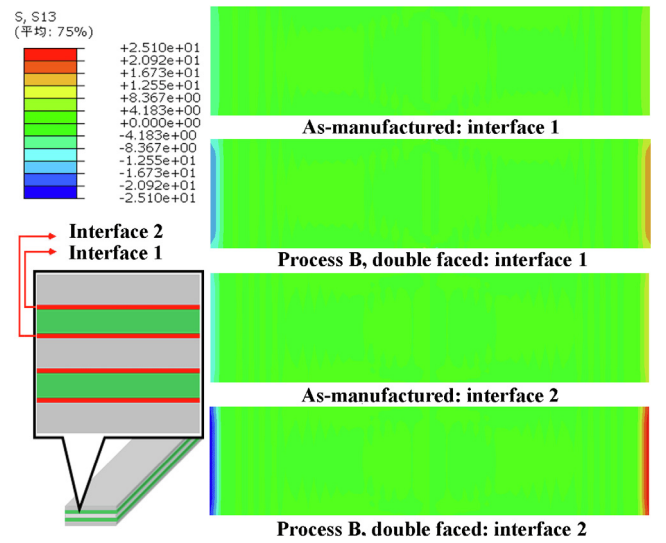
Fig. 8. interfacial shear stress of FMLs before and after shot peening.
