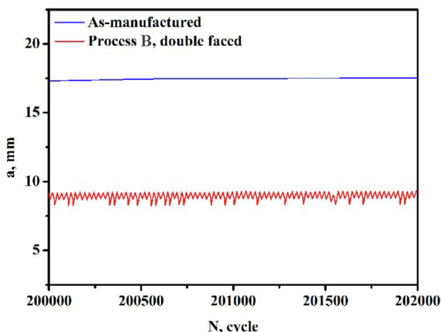
Fig. 16. Jagged a-N curve of shot peened FMLs.
