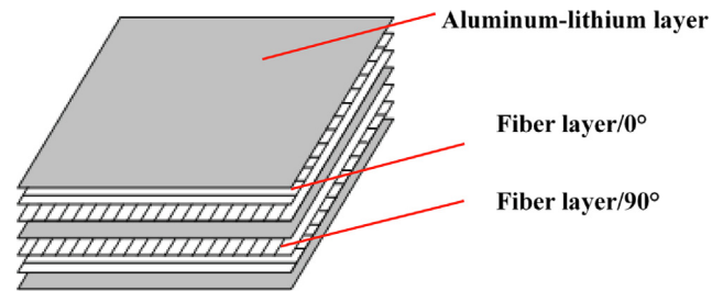
Fig. 1. The FMLs studied constitute an FML3-3/2-0.3 lay-up.
