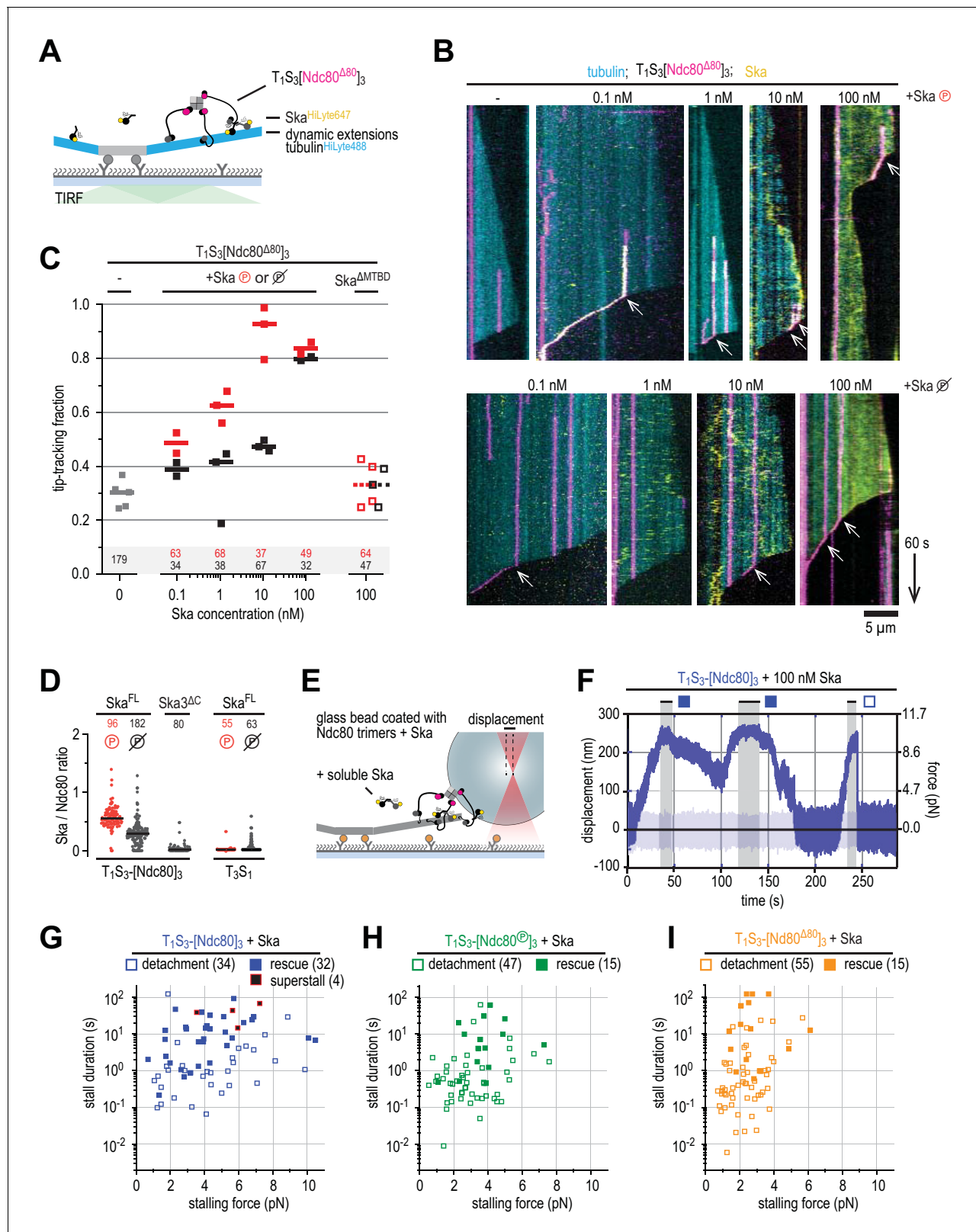
Figure 5. Ska bound to Ndc80 presents an additional microtubule end-binding site that stabilizes the stalled microtubule ends. (A) Ska and trimeric Ndc80 Δ80 modules were imaged simultaneously on dynamic microtubules using TIRF microscopy. (B) Trimeric Ndc80 Δ80 modules (magenta) on dynamic microtubules (cyan) in the presence of increasing concentrations of phosphorylated (top row) or dephosphorylated (bottom row) Ska (yellow). Scale bars: vertical (60 s), horizontal (5 μm). Arrows indicate successful end-tracking events. (C) Fraction of trimeric Ndc80 Δ80 modules that initiate movement Figure 5 continued on next page
