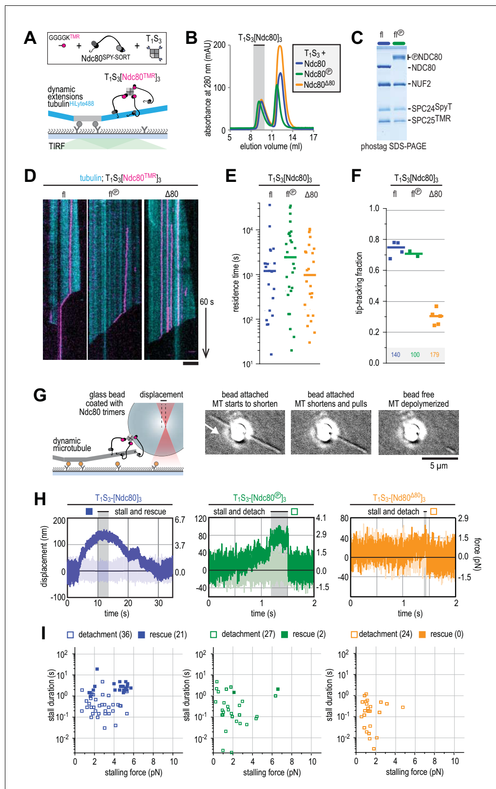
Figure 4. Ndc80-tail is required for interaction with a microtubule end. (A) Experimental setup featuring trimeric T 1 S 3 [Ndc80] 3 modules visualized on dynamic microtubules using TIRF microscopy. (B) Size-exclusion chromatography traces showing separation of monomeric Ndc80 from trivalent T 1 S 3 -Ndc80 modules using full-length Ndc80 (fl, blue), Aurora B phosphorylated full-length Ndc80 (fl-phosphorylated, green), and Δ80-Ndc80 (orange). (C) Phostag gel demonstrating successful phosphorylation of the NDC80 subunit by Aurora B. (D) Kymographs showing Ndc80 trimers (magenta) on Figure 4 continued on next page
