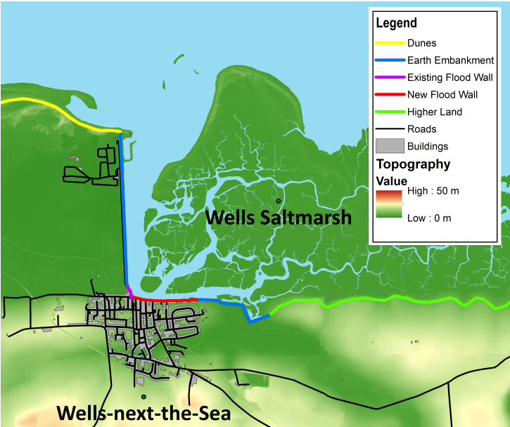
Figure 3.7: Current structural and natural coastal protection in Wells-next-the-Sea and possible flood wall extension.
