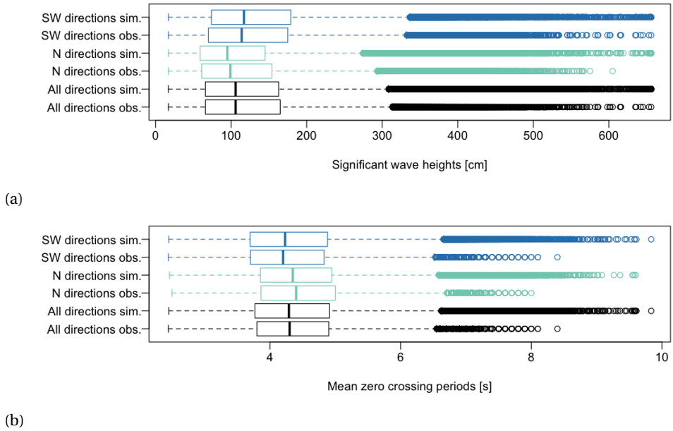
Figure 6.18: Boxplots of observed and simulated data for (a) significant wave height and (b) mean zero-crossing period.
