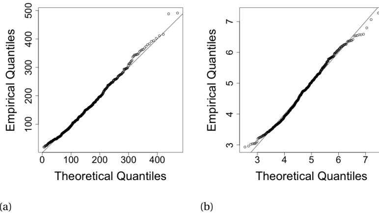
Figure 5.6: QQ-plots showing the fit of the univariate models for (a) significant wave heights and (b) mean zero-crossing periods
