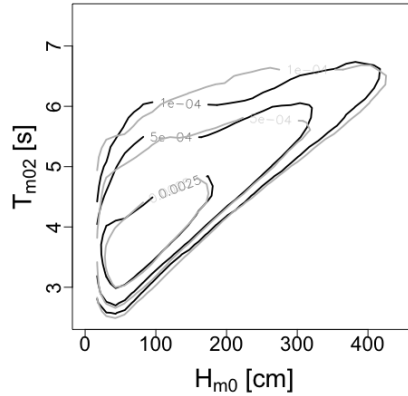
Figure 6.19: Bivariate density contours for significant wave heights and mean zero-crossing periods. Densities are estimated from 24 observed years (black) and 24 simulated years (gray).
