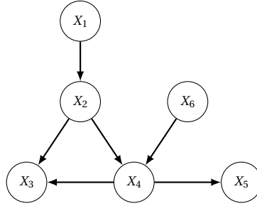
Figure 2.1: Example of a directed acyclic graph on six variables
