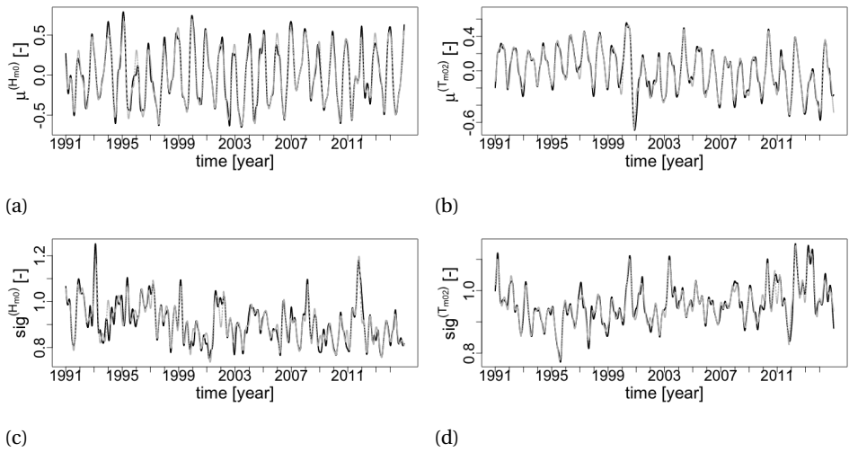
Figure 6.10: Seasonal mean and standard deviation processes: (a) \mu_t^{(Hm0)} , (b) \mu_t^{(Tm02)} , (c) \sigma_t^{(Hm0)} , and (d) \sigma_t^{(Tm02)} .
