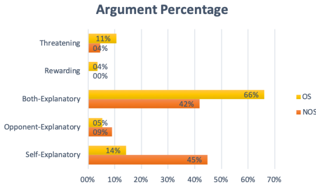
Figure 5: Argument Analysis
