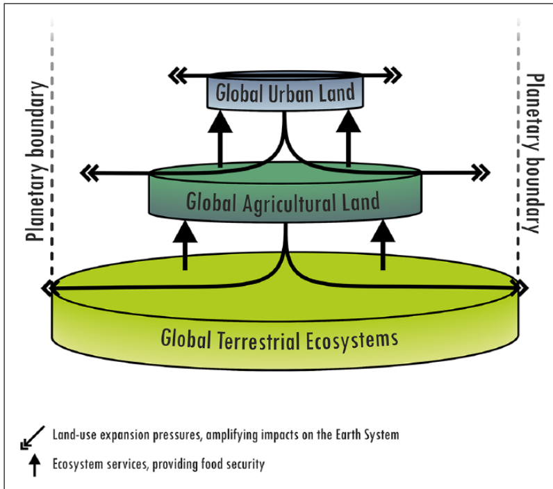
Figure 2. Urban and peri-urban soils are about twice as productive as the global average, and most of the global stock of land suitable for agriculture is already in use. Displacing crop production from urban and peri-urban land is expected to be mainly onto forest ecosystems with soils of lower productivity than the global average. In pursuit of food security, such displacement would require a substantially larger proportion of the Earth's terrestrial land surface than the surface area lost to urban encroachment, risking amplified impacts on the Earth System.
