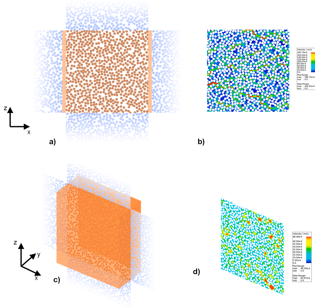
Fig. 3. Boundary conditions and corresponding flow fields in x- and y-directions (velocity magnitude), respectively. (a&c) Boundary conditions highlighting the implicit inlet/outlet voxels in orange and periodic tangential boundaries in blue. (b&d) velocity magnitude fields for the microstructure and boundary conditions shown in a&c.
