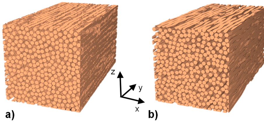
Fig. 1. a) EV generated by the original Monte-Carlo approach, b) EV generated without the short-range behavior. In both cases, r = 10 pixel, v_f = 0.6 .
