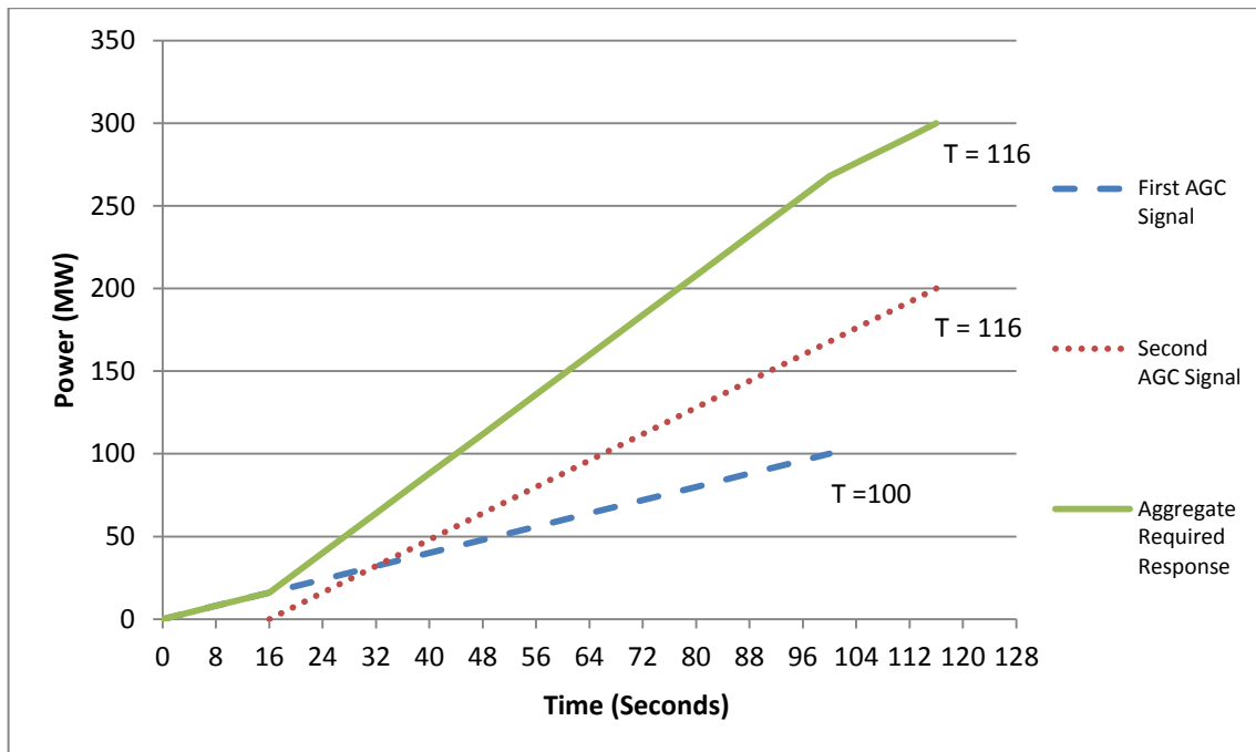
Figure 7: Secondary Reserves Response Example
