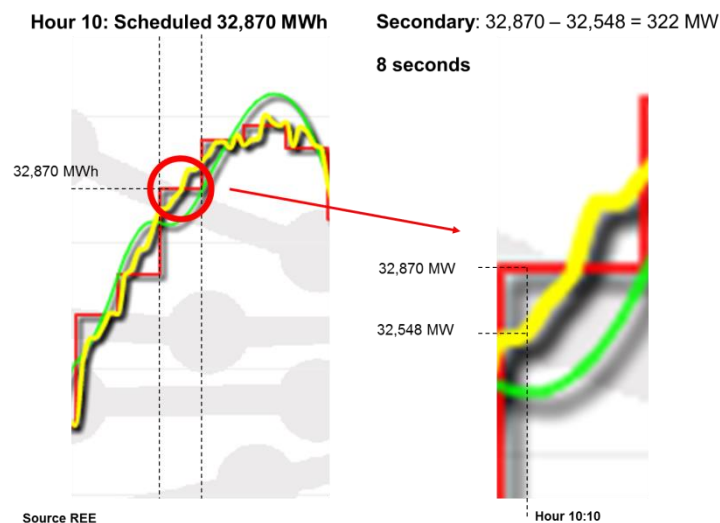
Figure 4: Close up of Real-time System Demand
