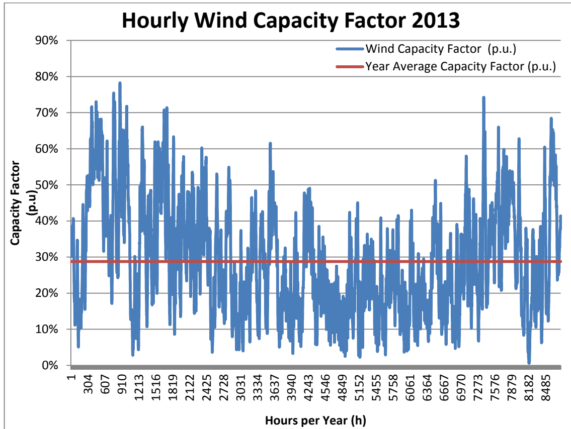
Figure 20: Hourly Wind Capacity Factor vs. Year Average Capacity Factor for MY2013
