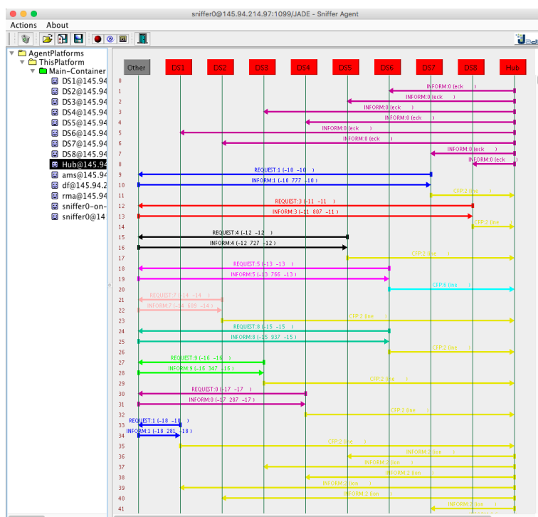
Figure 5.8: Single negotiation step shown in the Sniffer Agent in JADE
