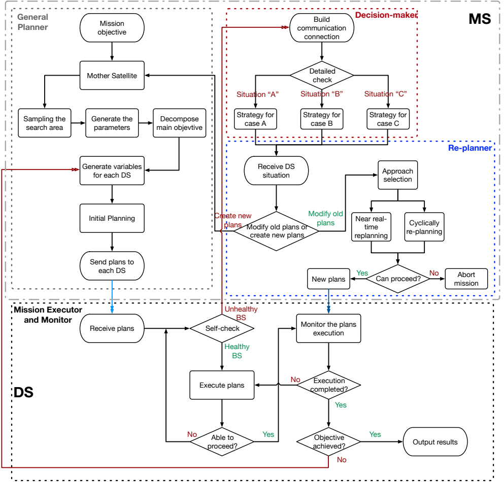
Figure 4.1: General flowchart of the planning and re-planning system for the reference MSS. It consists of four modules, the general planner (GP), the decision-maker (DM), the re-planner (RP), and DS mission executor and monitor (MEM). The GP, DM and RP are located on the MS, and the MEM is located on each DS.
