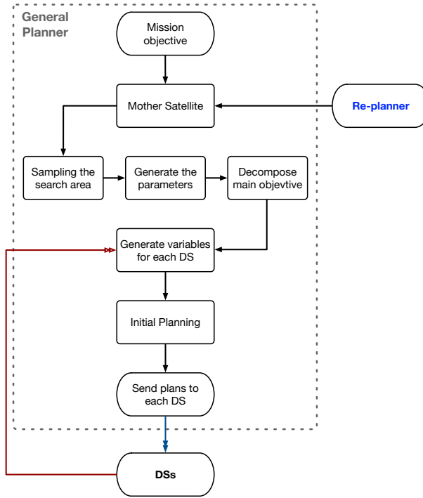
Figure 4.2: Flowchart of the general mission planner
