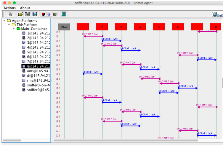
Figure 5.13: BBP negotiation
