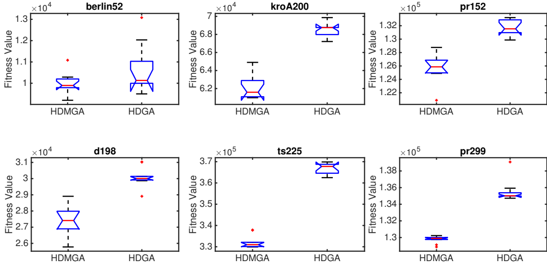
Figure 6.4: Fitness value on six study cases for HDMGA and HDGA approaches
