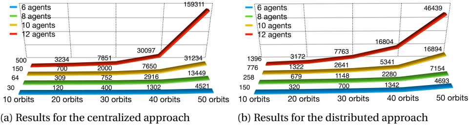
Figure 6.7: Average computation time comparison for centralized and distributed approaches to solve five mission objectives using four different team sizes
