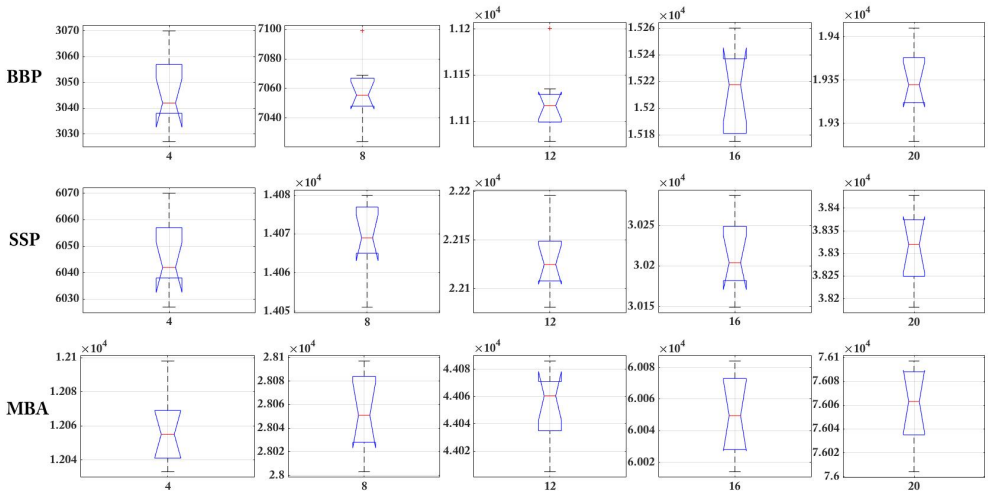
Figure 5.14: Statistical results of CPU time for three negotiation mechanisms (BBP, SSP and MBA)
