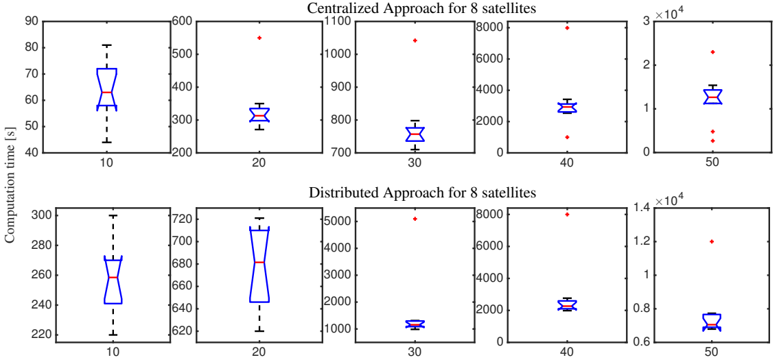
Figure 6.6: Computation time on 8 satellites for both approaches
