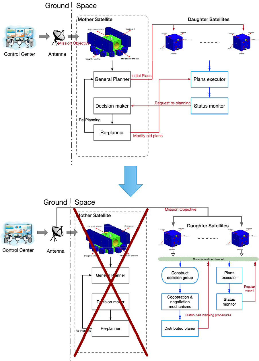
Figure 6.1: Organizational architecture change due to the loss of the main controller
