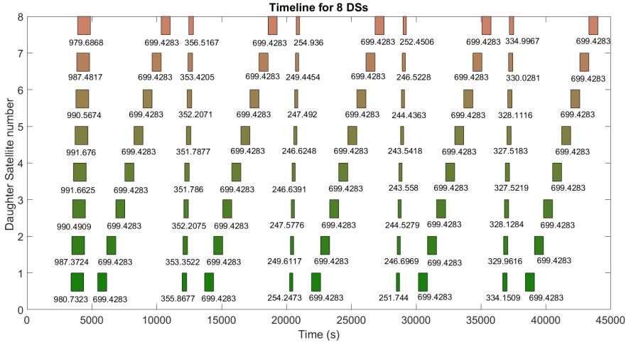
Figure 3.9: Initial planning sequences for eight DSs over five orbits. Each DS in each orbit has two behaviors, the frontier one represents the observation and the later one stands for the communication window. The parameters under each box represent the corresponding duration of each behavior.
