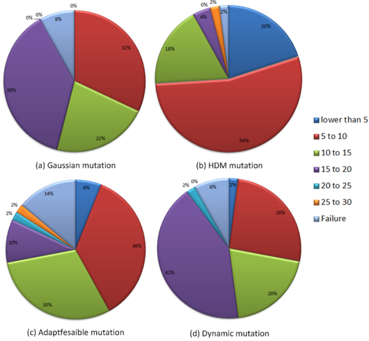
Figure 3.7: Data distribution based on computation time over the 50 simulations
