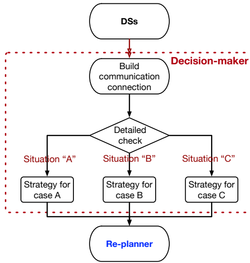
Figure 4.4: Flowchart of the decision-maker
