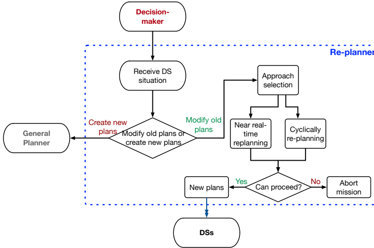
Figure 4.5: Flowchart of the re-planner
