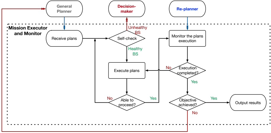
Figure 4.3: Flowchart of the mission executor and monitor for each DS
