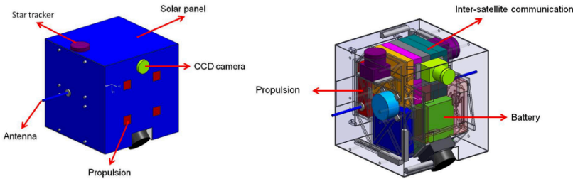
Figure 2.3: Daughter satellite with examples of parts of onboard sub-systems: star trackers, propulsion system, inter-satellite antenna, solar cells, and battery (these two figures are taken from [Boonstra et al., 2016]).
