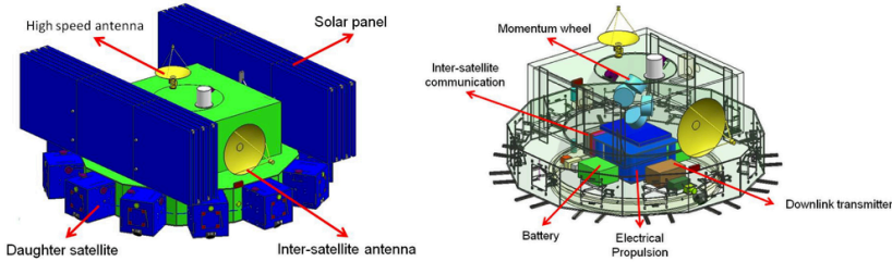
Figure 2.2: Mother satellite with examples of parts of onboard sub-systems, including stowed antennas, daughter satellites, solar panels, momentum wheel, battery, and propulsion system (these two figures are taken from [Boonstra et al., 2016]).
