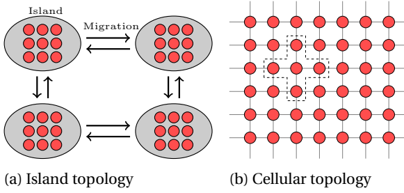
Figure 1.4: Sample topologies for multi-agent systems
