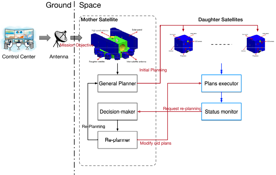
Figure 3.1: General architecture of controlling the centralized MSS
