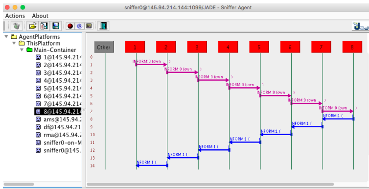
Figure 5.12: SSP negotiation
