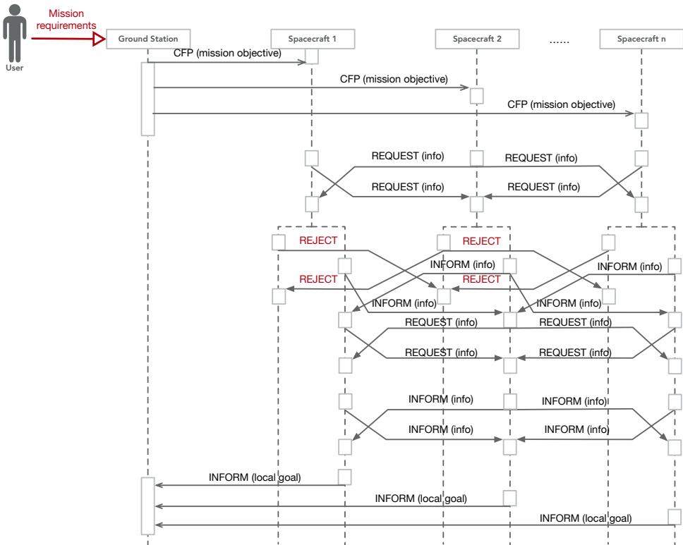
Figure 5.6: Broadcast-based Play
