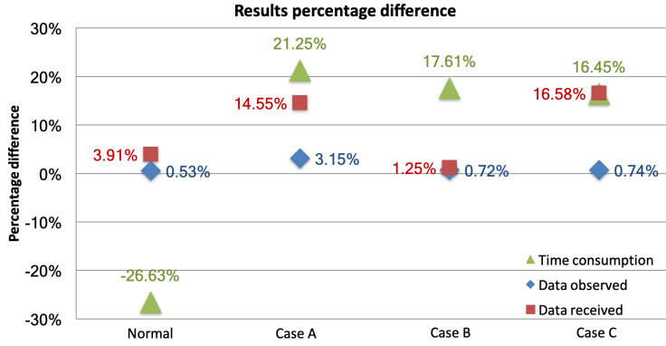
Figure 4.15: Percentage differences of CRM and NRRM on three aspects for various cases
