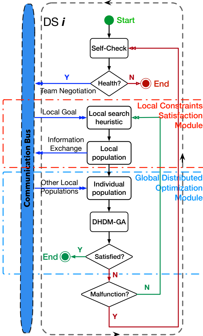
Figure 6.2: Flow chart of HDGA for each satellite
