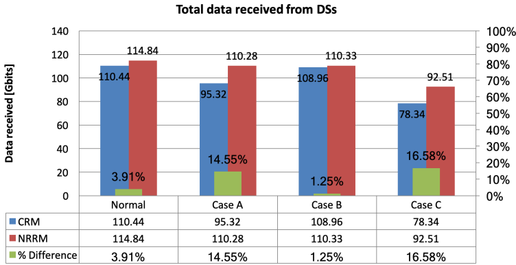
Figure 4.13: The number of data received by the MS for the normal case, and the three emergency cases within a certain lifetime
