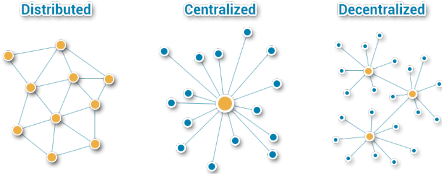
Figure 2.5: Three organizational architectures: The one in the middle is the centralized architecture, which has a single controller to control all the nodes; The one on the left is the distributed architecture, where all the nodes are equivalent and are connected; The one on the right is the decentralized architecture, where each node is only connected with its neighbors. (This figure is adopted from [Quantalysus, 2018])
