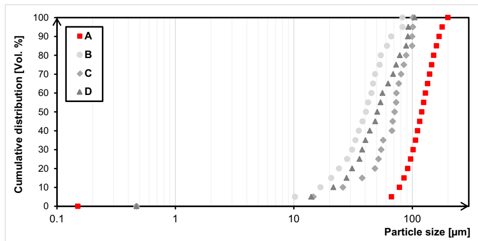
Fig. 7. Cumulative particle size distributions of river sand and fRCA, 0–0.250 mm, analyzed by laser diffraction using ethanol as dispersion medium.
