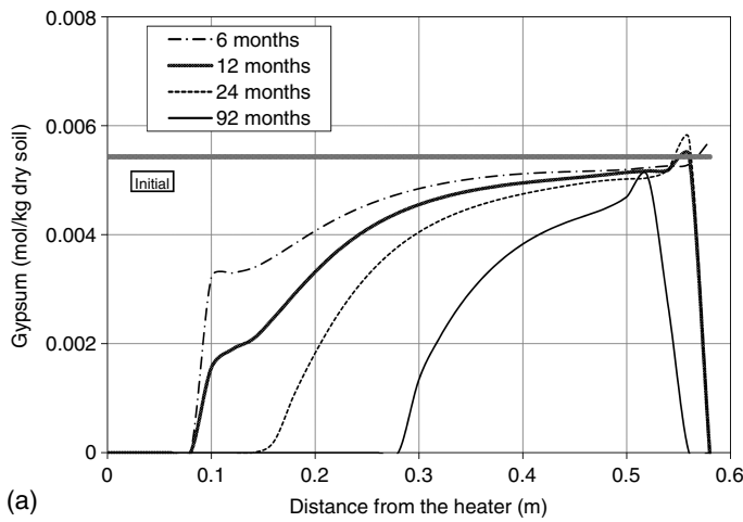
Fig. 8. Variations of (a) gypsum; and (b) anhydrite in the domain obtained from the transient analysis.
