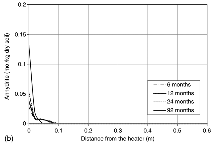
Fig. 8. Variations of (a) gypsum; and (b) anhydrite in the domain obtained from the transient analysis.
