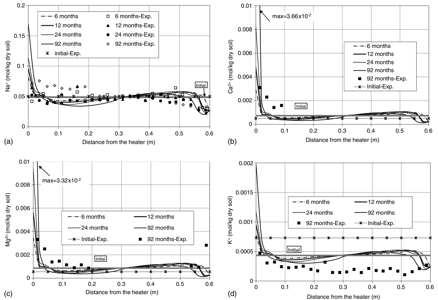
Fig. 13. Variations of (a) sodium; (b) calcium; (c) magnesium; and (d) potassium ions obtained by the postmortem analysis and experiments. (Experimental data from Fernández and Villar 2010.)
