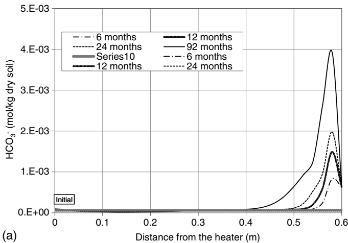
Fig. 9. Variations of bicarbonate in the domain obtained from the (a) transient analysis; and (b) postmortem analysis (experimental data from Fernández and Villar 2010).
