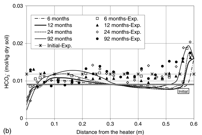
Fig. 9. Variations of bicarbonate in the domain obtained from the (a) transient analysis; and (b) postmortem analysis (experimental data from Fernández and Villar 2010).
