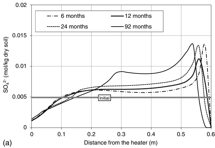
Fig. 7. Variations of sulfate in the domain obtained from the (a) transient analysis; and (b) postmortem analysis (experimental data from Fernández and Villar 2010).
